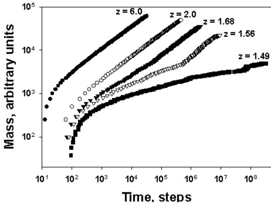
Figure 2. Simulation of cumulative imbibition over a range of pore coordinations.
