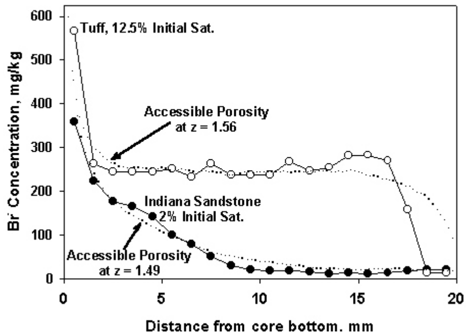
Figure 5. Concentration profiles of bromide following imbibition into welded tuff (12.5% initial
