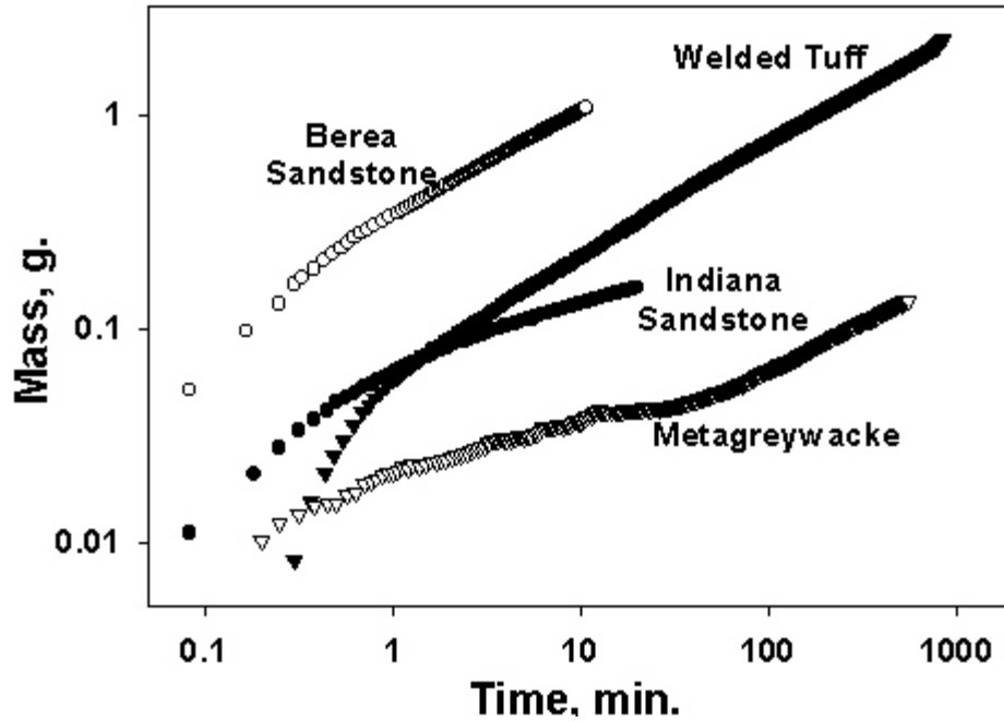
Figure 1. Experimental results showing cumulative imbibition into Berea sandstone, Indiana sandstone, welded tuff, and metagraywacke.
