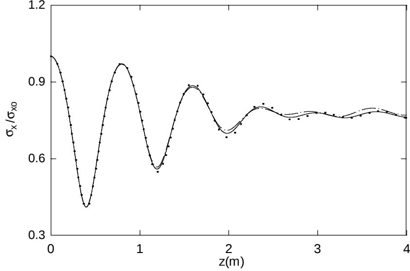
Figure 3.22: Comparison of results for the evolution of the rms beam size of the initially gaussian beam with \alpha = 5 obtained using \Delta = 12 ( - \cdot - ), \Delta = 10 ( — ) and \Delta = 8 ( \cdot \cdot \cdot ).
