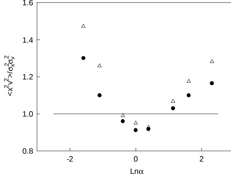
Figure 3.16: Comparison of the dynamical CME results (●) and PIC predictions (△) for the correlation ratio \langle x^2 v_x^2 \rangle / (\sigma_x^2 \sigma_v^2) of the initially gaussian beam vs the initial mismatch \alpha . The solid line corresponds to a fully thermalized beam and is plotted for a reference.
