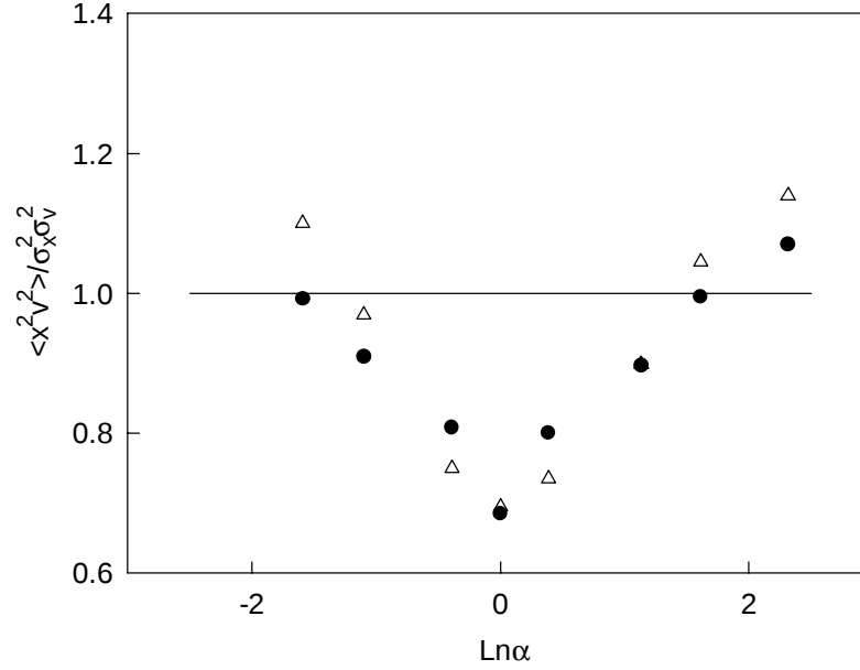
Figure 3.17: Comparison of the dynamical CME results (●) and PIC predictions (△) for the correlation ratio \langle x^2 v_x^2 \rangle / (\sigma_x^2 \sigma_v^2) of the initially uniform beam vs the initial mismatch \alpha . The solid line corresponds to a fully thermalized beam and is plotted for a reference.
