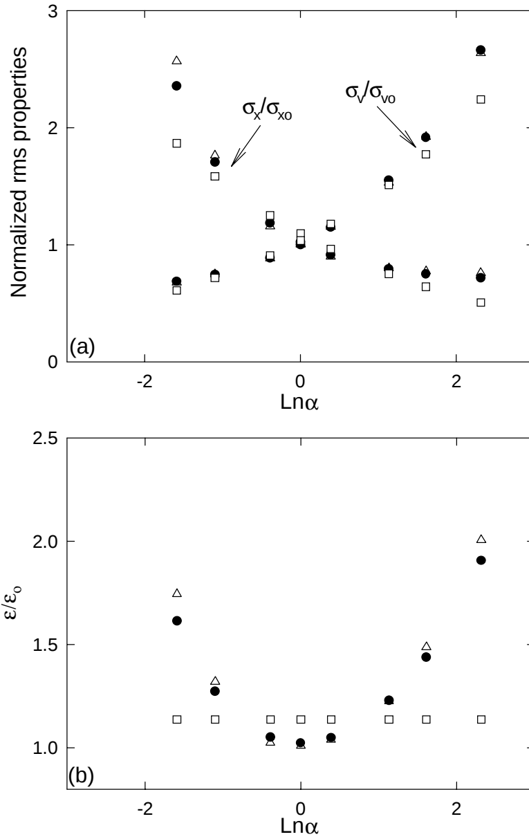
Figure 2.4: Comparison between the new analytical predictions ( \bullet ) given by Eqs. (2.33), (2.38) and (2.40), predictions of Ref. [1] ( \square ) given by Eqs. (2.13)-(2.15) and PIC results ( \triangle ) for (a) the rms beam properties and (b) the emittance vs the initial mismatch \alpha of the initially gaussian beam.
