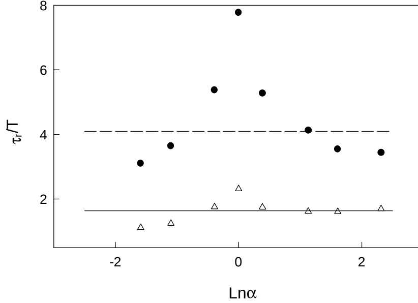
Figure 4.12: Comparison of PIC results for the relaxation time with the estimates of Eqs. (4.18) (—) and (4.19) (- - -) for initially gaussian ( \triangle ) and uniform ( \bullet ) beams.
