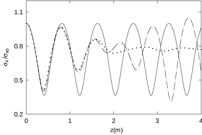
Figure 3.1: Comparison of results for the evolution of the rms beam size obtained by a PIC simulation ( \cdot \cdot \cdot ) and by a CME integration with different truncation orders j_{max} = 2 (—) and j_{max} = 4 ( - \cdot - ).
