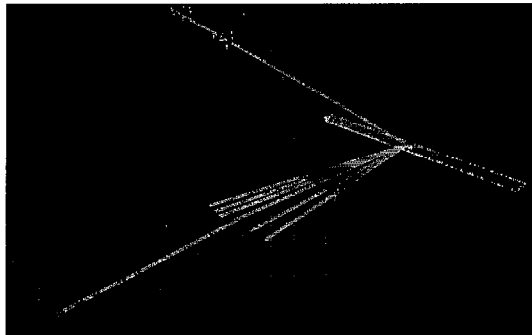
Figure 2d: A Au+Au RHIC collision at s^{1/2} = 200 GeV recorded by the BRAHMS experiment. Each line represents a particle.
