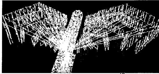
Figure 2c: A Au+Au RHIC collision at s^{1/2} = 200 GeV recorded by the PHOBOS experiment. Each line and dot represents a particle.
