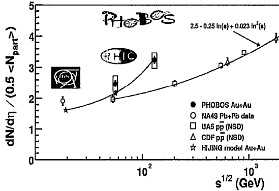
Figure 5: The charged particle multiplicity normalized to the number of participants in the collision as a function of s^{1/2} . Shown are results from the SPS (NA49) and RHIC (PHOBOS). The curve on the left shows predictions from the HIJING simulation. The points and curve on the right are measurements of the baseline nucleon-nucleon collisions (UA5 and CDF).
