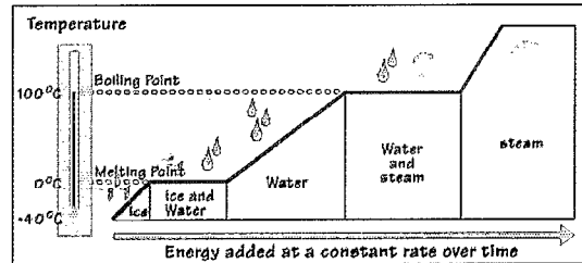
Figure 8: The heating curve for ice to steam showing that the temperature remains constant when the system is undergoing a phase transition.
