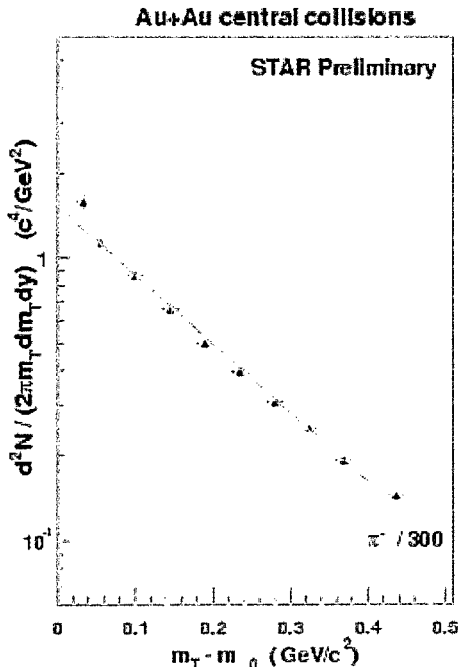
Figure 7: The transverse mass distribution (with the pion rest mass subtracted) for negatively charged pions as measured by the STAR experiment in the 5% most central collisions. The solid lines are fits performed as described in the text.
