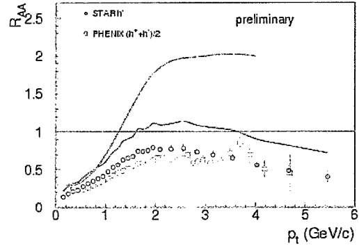
Figure 13: The ratio of the number of charged particles measured in central nucleus-nucleus collisions to that measured in nucleon-nucleon collisions as a function of transverse momentum as measured by PHENIX and STAR at RHIC. At high p_t , where jet processes occur, the ratio is low and decreasing with increasing p_t . This behavior is consistent with jet suppression by a QGP, but it is still too early to know this for sure.
