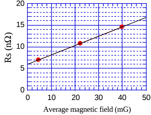
Figure 8: Residual resistance as a function of magnetic field averaged over 5 cells. The sensitivity is calculated to be 0.22 n \Omega /mG.
