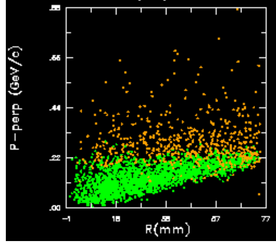
Figure 1: p_r versus r projection at z = 0 of macroparticles that survive to z = 35 m (green dots) and those which are lost (orange dots).
