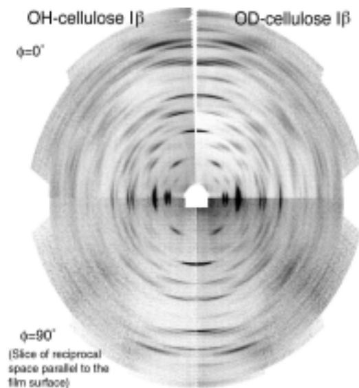
Figure 1 , Neutron diffraction data collected on D19 at the ILL, Grenoble, France, from cellulose I \beta . The image has been remapped into cylindrical reciprocal space with the fiber axis vertical. The left-hand side corresponds to hydrogenated cellulose and the right-hand side to deuterated cellulose.
