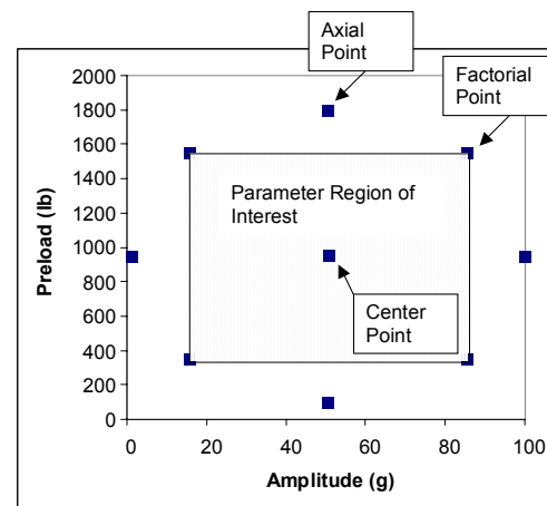
Figure 6: Example of a Central Composite Design for 2 Parameters
