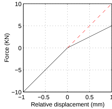
Figure 3: Damage simulation using a bilinear stiffness model
