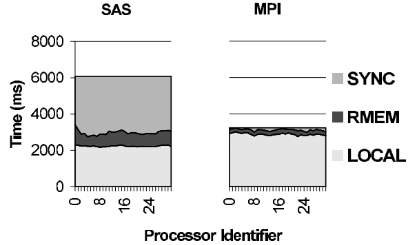
Figure 6. N-BODY time breakdown for SAS and MPI on 32 processors for 128K particles.
