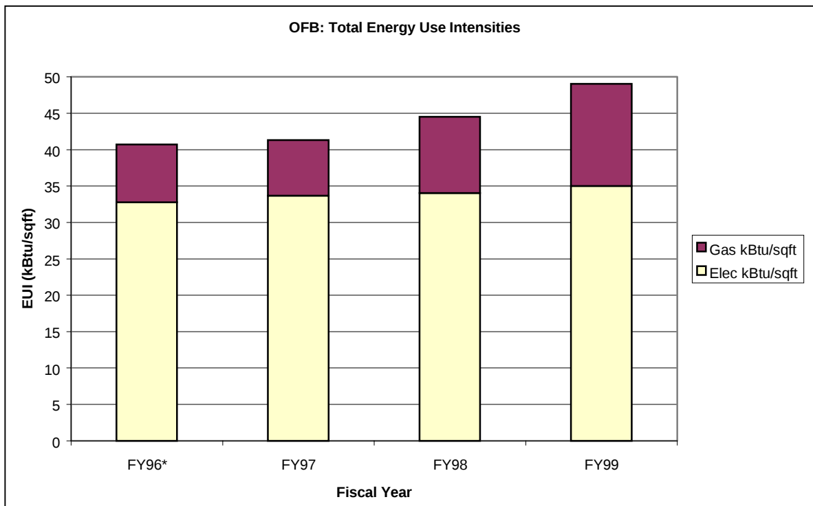
Figure 1: Multi-year whole-building site energy use at the Oakland Federal Building.
