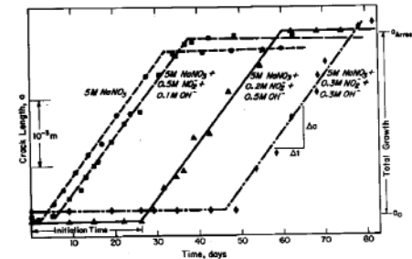
FIGURE 11. Crack Length as a Function of Time 18
