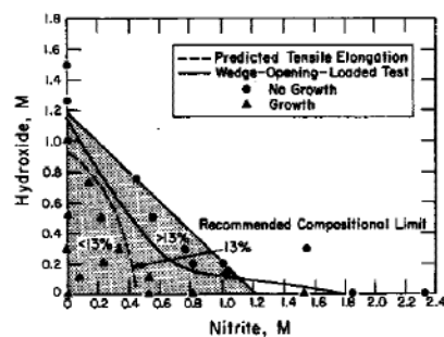
FIGURE 15. Comparison of Electrochemical Tensile Test With Wedge-Opening-Loaded Specimens in 5M NaNO 3 , at 97°C
