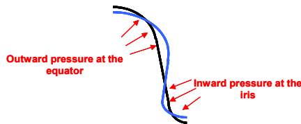
Figure 1: Lorentz pressures.
