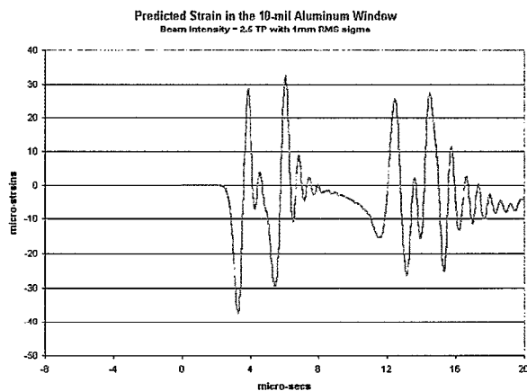
Figure 4. Predicted strains (ANSYS) in the 10mil aluminum window for 2.5 TP and 1mm sigma
