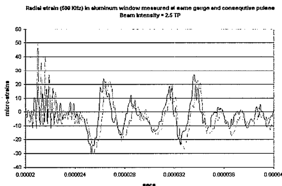
Figure 5. Strain in aluminum window recorded by the same strain gauge and back-to-back pulses
