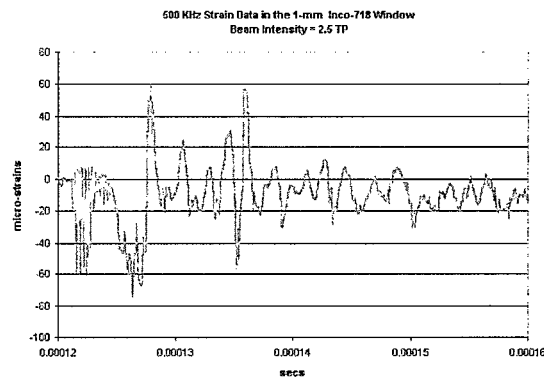
Figure 6. Measured strains in a 1mm Inconel window
