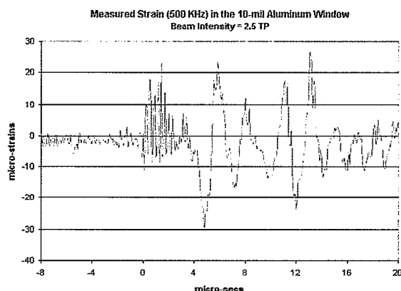
Figure 3. Radial strain measured in the 10mil aluminum window and induced by a 2.5 TP beam with 1mm sigma
