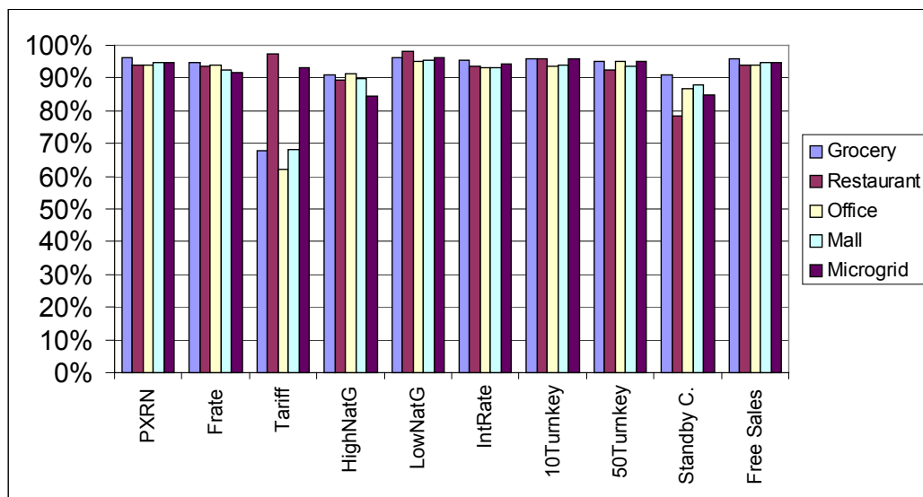
Figure 7. Percent Coverage of Energy Consumption through Installed DER Capacity
