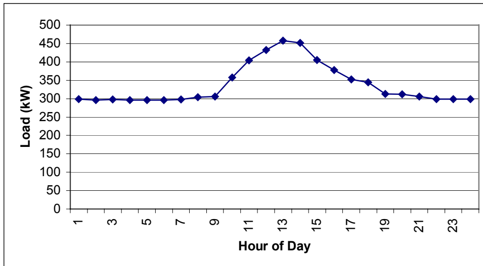
Figure 2. August Peak Day Load Profile for Grocery
