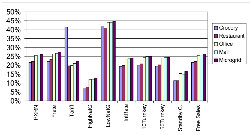
Figure 5. Savings Over a "Do-Nothing" Case
