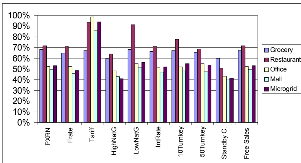
Figure 6. Percent Coverage of Peak Demand through Installed Capacity
