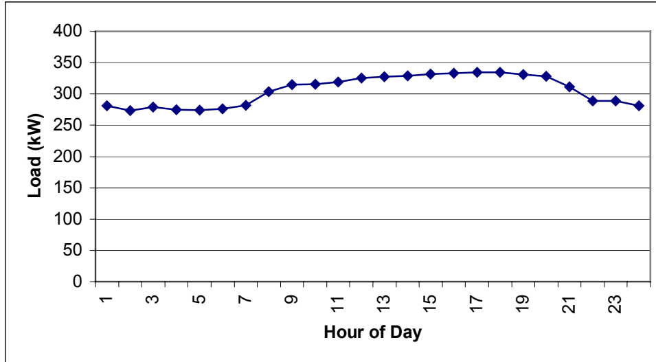
Figure 1. January Peak Day Load Profile for Grocery
