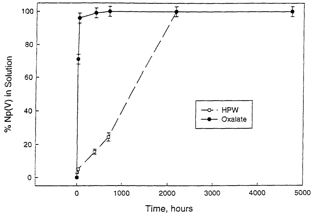
Figure 3. Buildup of Np(V) as a Function of Time due to Reduction in the Low Ionic Strength Organic Experiments. Reduction for Citrate and EDTA (not shown) was Instantaneous.
