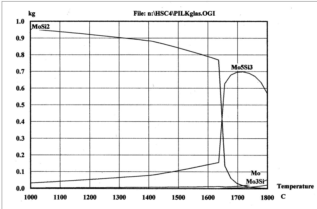
Figure 7: Thermodynamic equilibrium calculation of MoSi 2 in the LOF-Pilkington glass composition, as a function of temperature.
