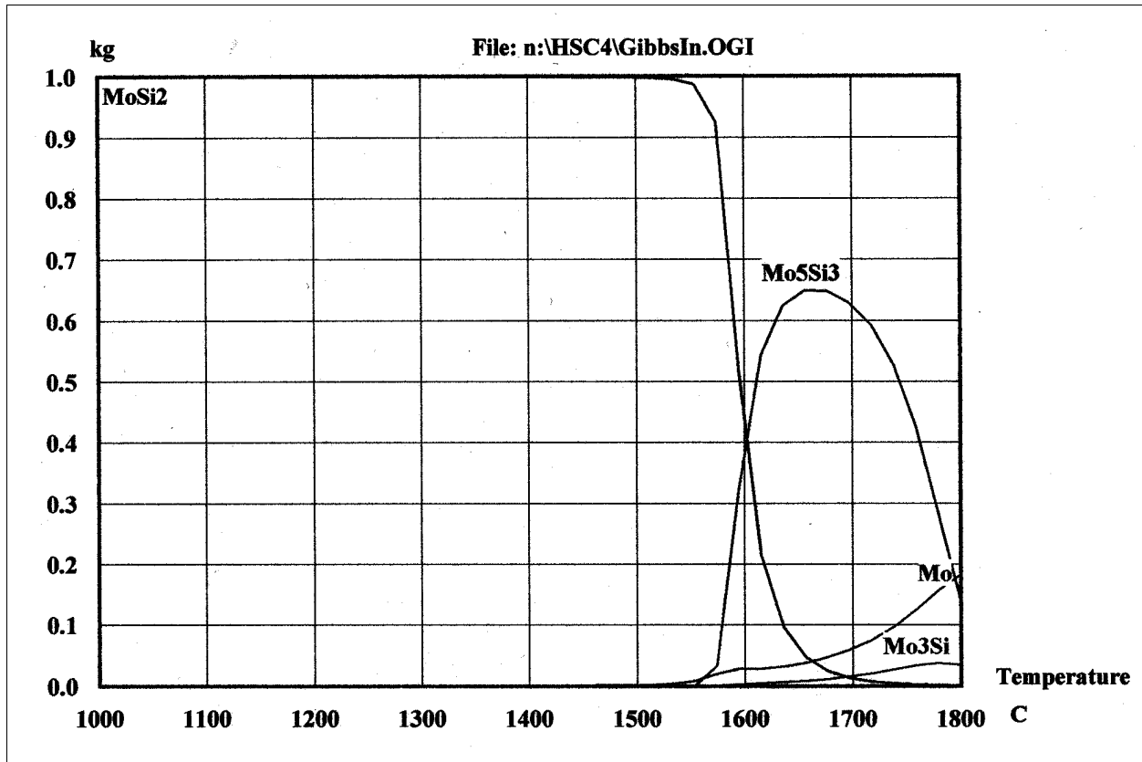
Figure 5: Thermodynamic analysis of equilibrium stability of MoSi 2 in TCE Panel Glass composition, as a function of temperature.
