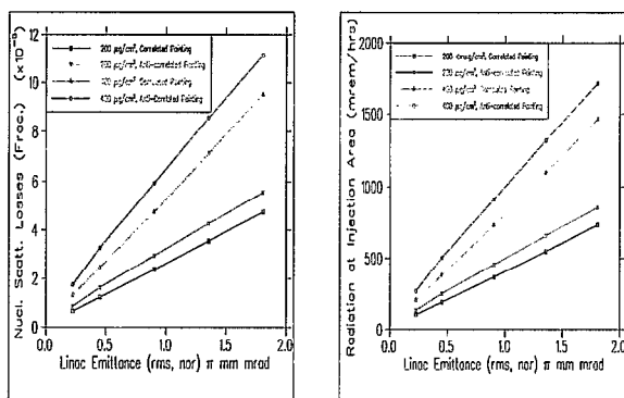
Figure 6 (a) Fractional beam losses at injection area and (b) radiation level due to nuclear scattering in the stripping foil as functions of normalized RMS emittance of injected beam [6].
