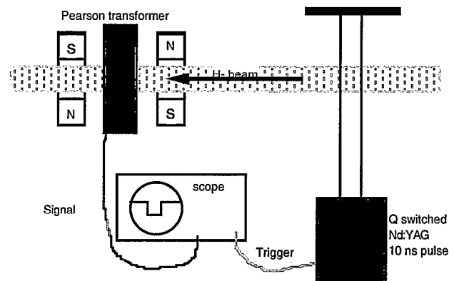
Figure 2: Laser scanner experiment on BNL linac. The first of two 10 Gm dipole magnets removes the free electrons from the beam and the second straightens the beam.
