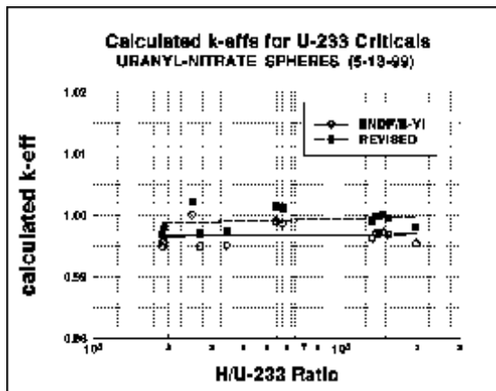
Figure 1. Calculated K-effs for uranyl-nitrate spheres.
