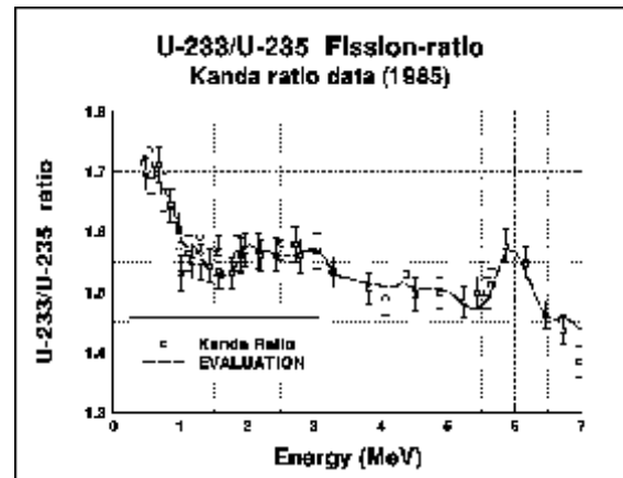
Figure 5. U-233/U-235 fission-ratio.
