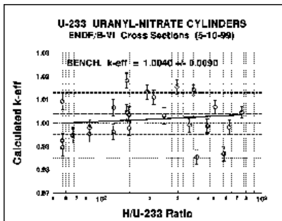
Figure 3. Uranyl-nitrate cylinders, ENDF/B-VI evaluation.
