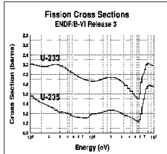
Figure 4. U-233 and U-235 fission cross-sections.
