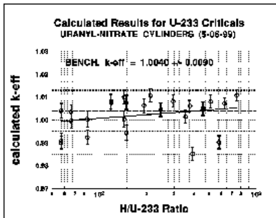
Figure 2. Uranyl-nitrate cylinders, revised evaluation.
