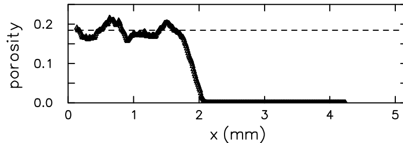
Figure 4. Intermediate, compaction wave with precursor. Piston velocity of 500 m/s and time of 1.6 \mu s. (a) The black region on the right indicated the distance the piston has traveled, and the solid lines represent interfaces of the grains. (b) Dashed lines correspond to minimum and maximum values. (c) Dashed line represents the initial porosity.
