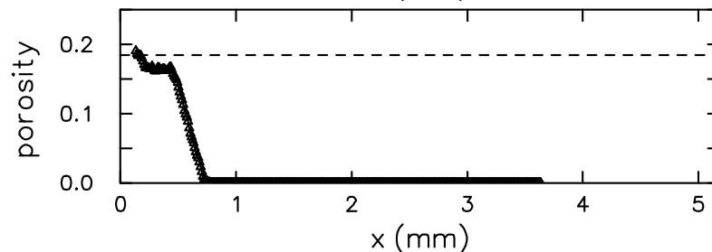
Figure 7. Strong, shock-like compaction wave. Piston velocity of 1000 m/s and time of 1.4 \mu\text{s} . (a) The black region on the right indicated the distance the piston has traveled, and the solid lines represent interfaces of the grains. (b) Dashed lines correspond to minimum and maximum values. (c) Dashed line represents the initial porosity.
