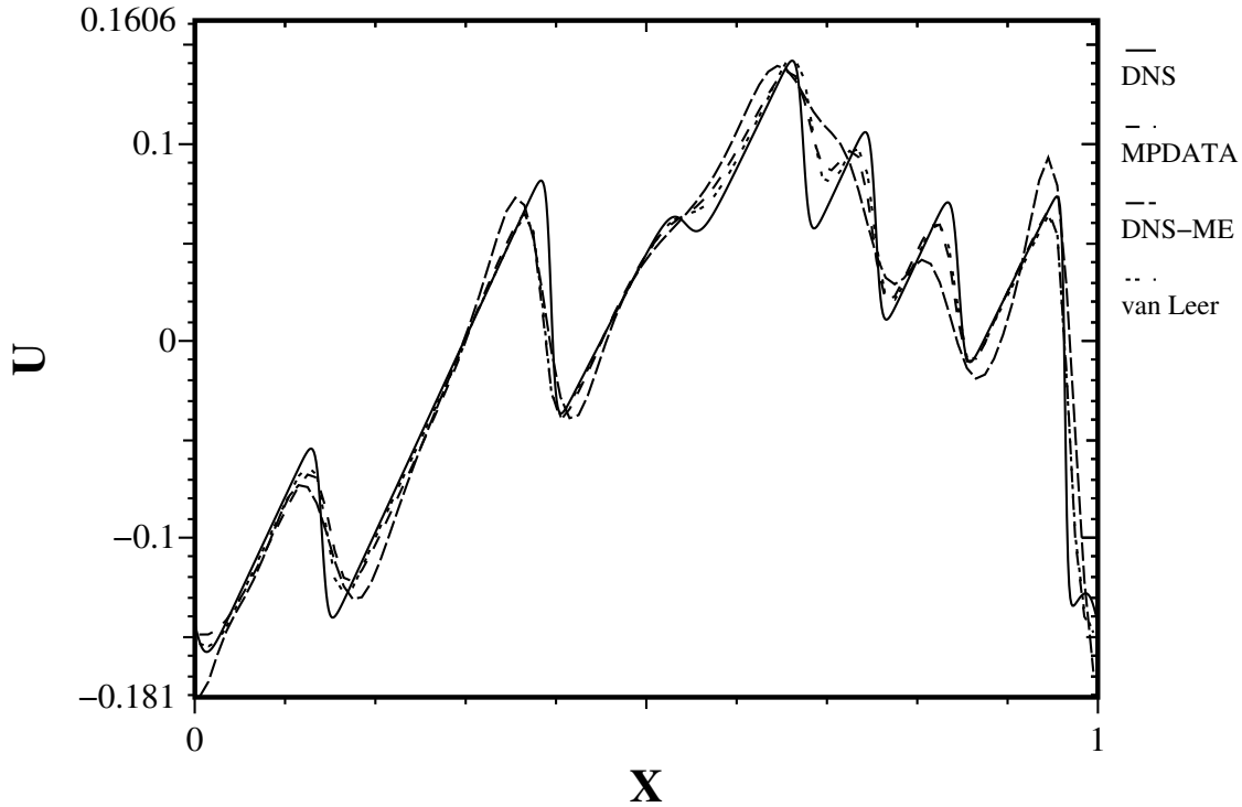
Figure 7: A comparison of the multimode solutions at t = 1.0 with a larger viscosity, \lambda_2 = 0.0002 , for DNS and several LES alternatives.
