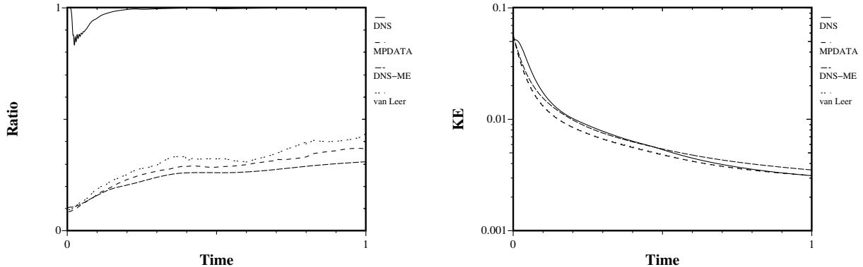
Figure 8: A comparison of the multimode solution’s kinetic energy decay with a larger viscosity, \lambda_2 = 0.0002 , for DNS and several LES alternatives.
