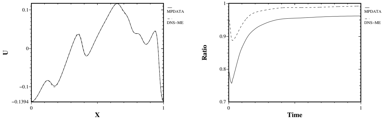
Figure 2: Comparing the final solutions for the multimode random sine wave using MPDATA and the DNS-ME for high viscosity \lambda = 0.001 . The right figure compares the time histories of the ratio of the viscous and the total energy dissipation rates from MPDATA and the DNS-ME for high viscosity.
