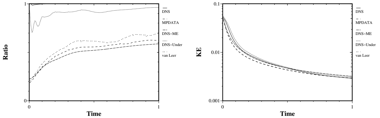
Figure 6: A comparison of the multimode solution's kinetic energy decay with a larger viscosity, \lambda_1 = 0.0005 , for DNS and several LES alternatives.
