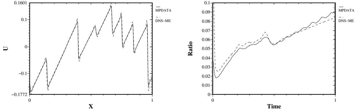
Figure 3: The final solution for the multimode random sine wave using MPDATA and the DNS-ME for low viscosity \lambda = 0.00001 . The right figure compares the time histories of the ratio of the viscous and the total energy dissipation rates from MPDATA and the DNS-ME for low viscosity.
