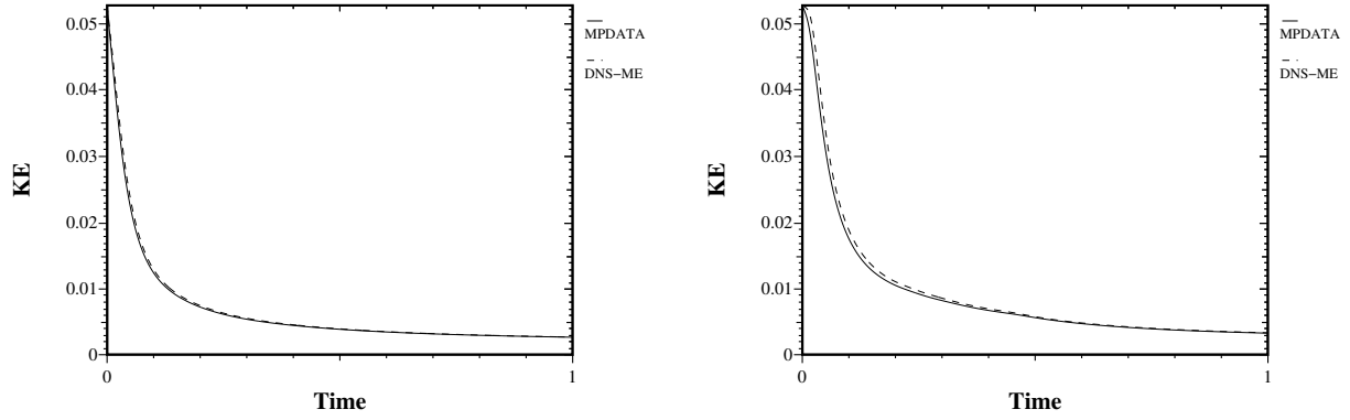
Figure 4: Comparing the kinetic energy histories for the high viscosity (left panel) and low viscosity (right panel) cases. The modified equation closely reproduces the MPDATA dissipation but is very slightly less dissipative.
