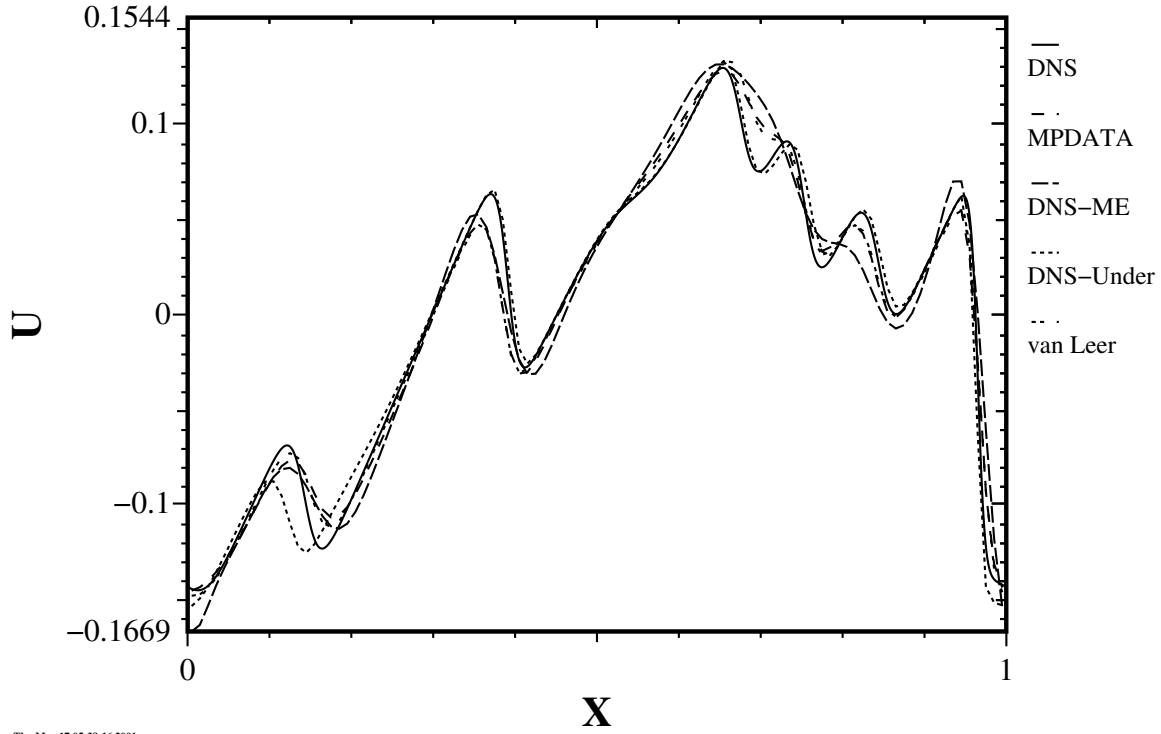
Figure 5: A comparison of the multimode solutions at t = 1.0 with a larger viscosity, \lambda_1 = 0.0005 , for DNS and several LES alternatives.
