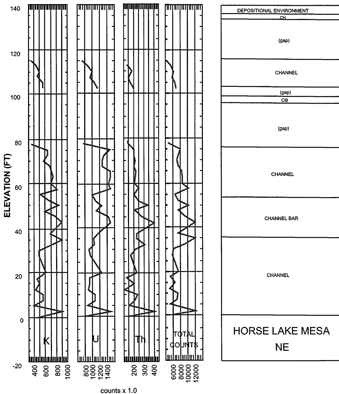
Figure 5: Composite GAD-6 gamma-ray spectrometer data for section 7: Horse Lake Mesa NE.
