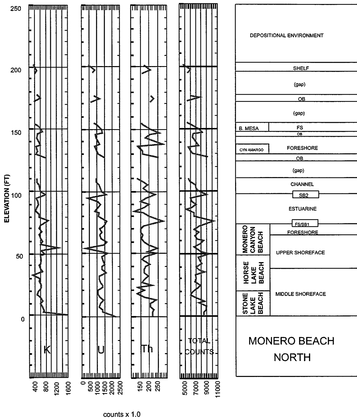
Figure 8: Composite GAD-6 gamma-ray spectrometer data for section 12: Monero Beach North.
