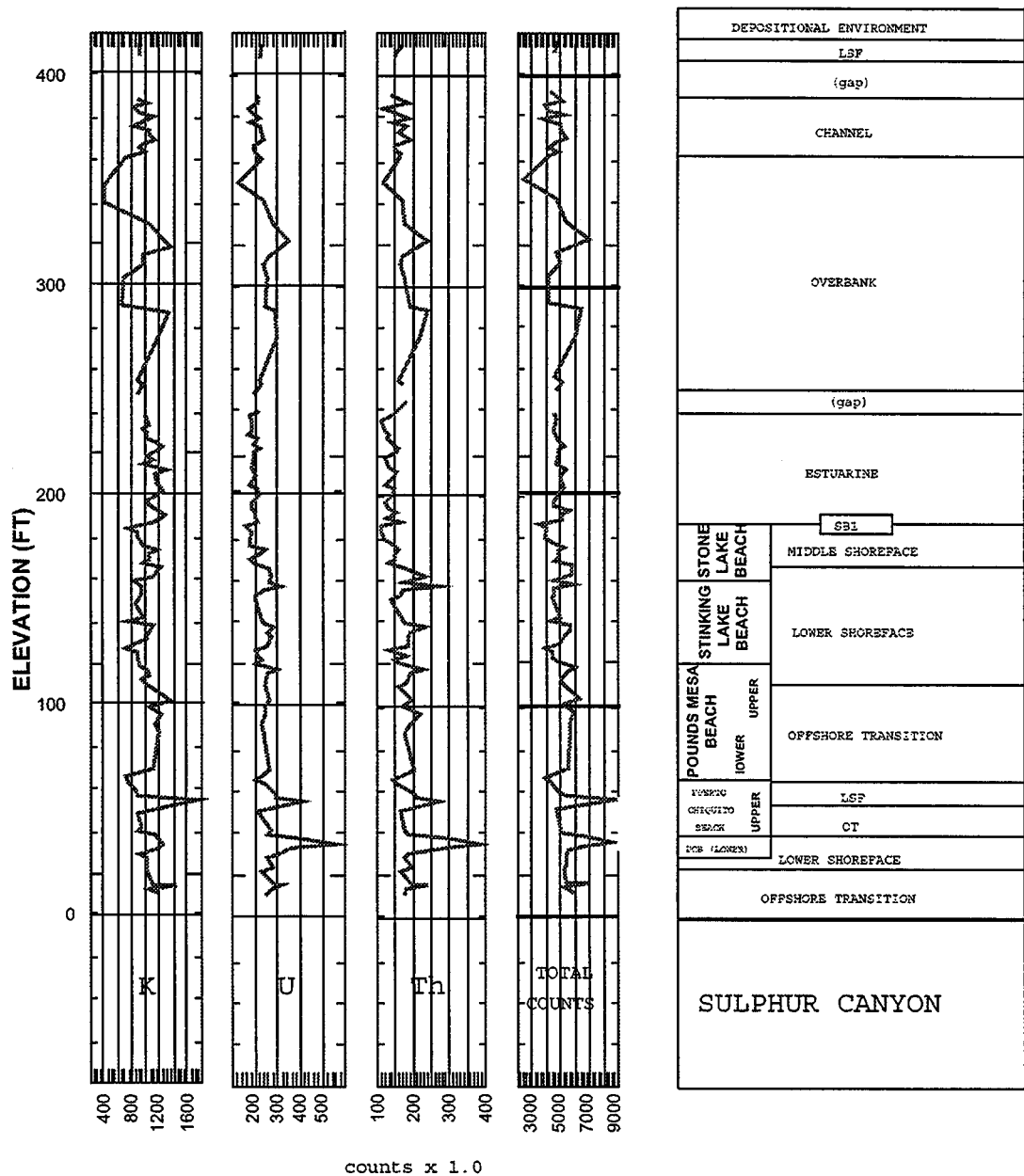
Figure 6: Composite GAD-6 gamma-ray spectrometer data for section 9: Sulphur Canyon.
