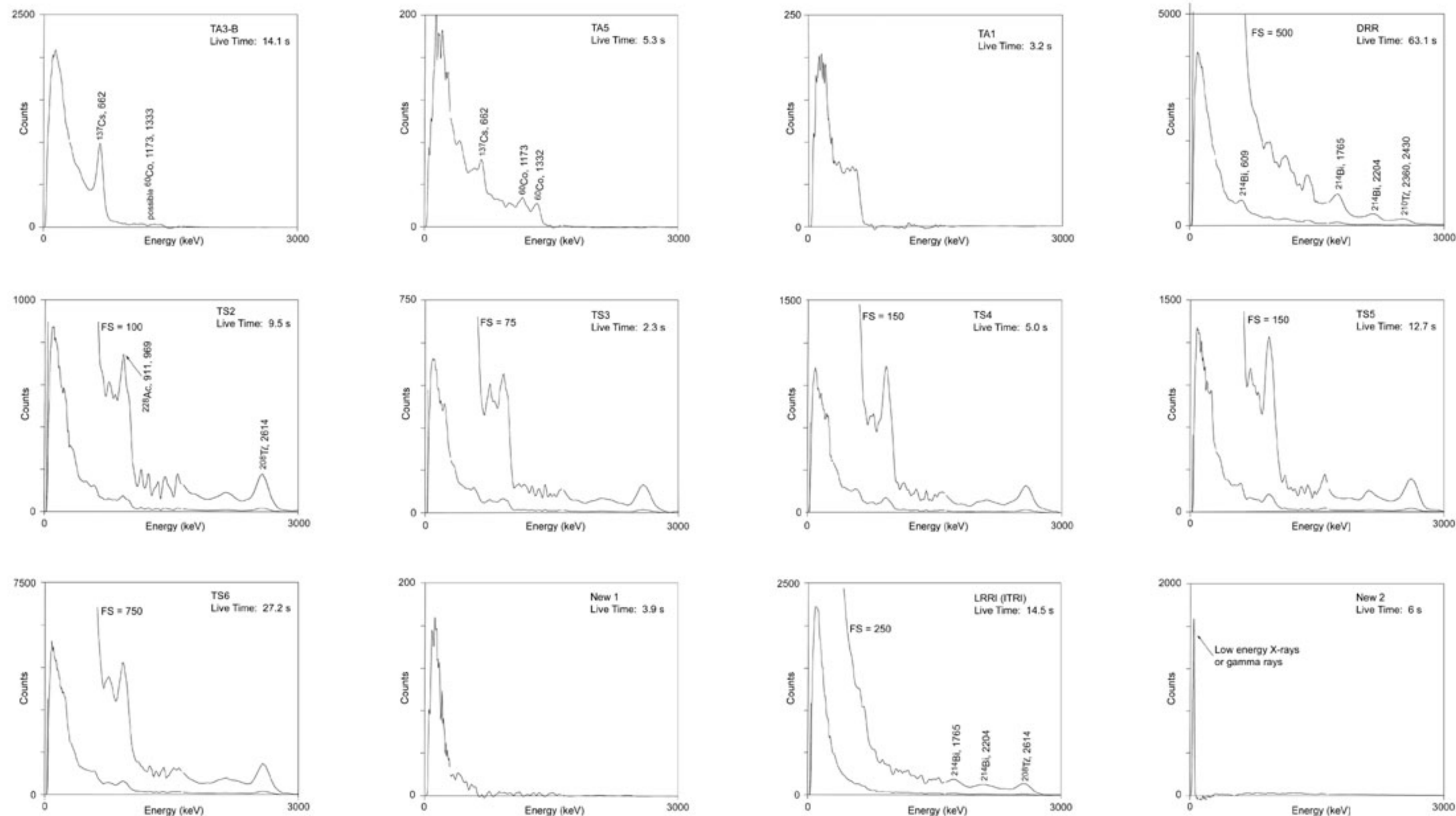
FIGURE 8. NET SPECTRA FROM AREAS SHOWN IN FIGURE 7. The net spectra were formed by subtracting a background spectrum from a high-activity spectrum generated from the areas labeled in Figure 7.
