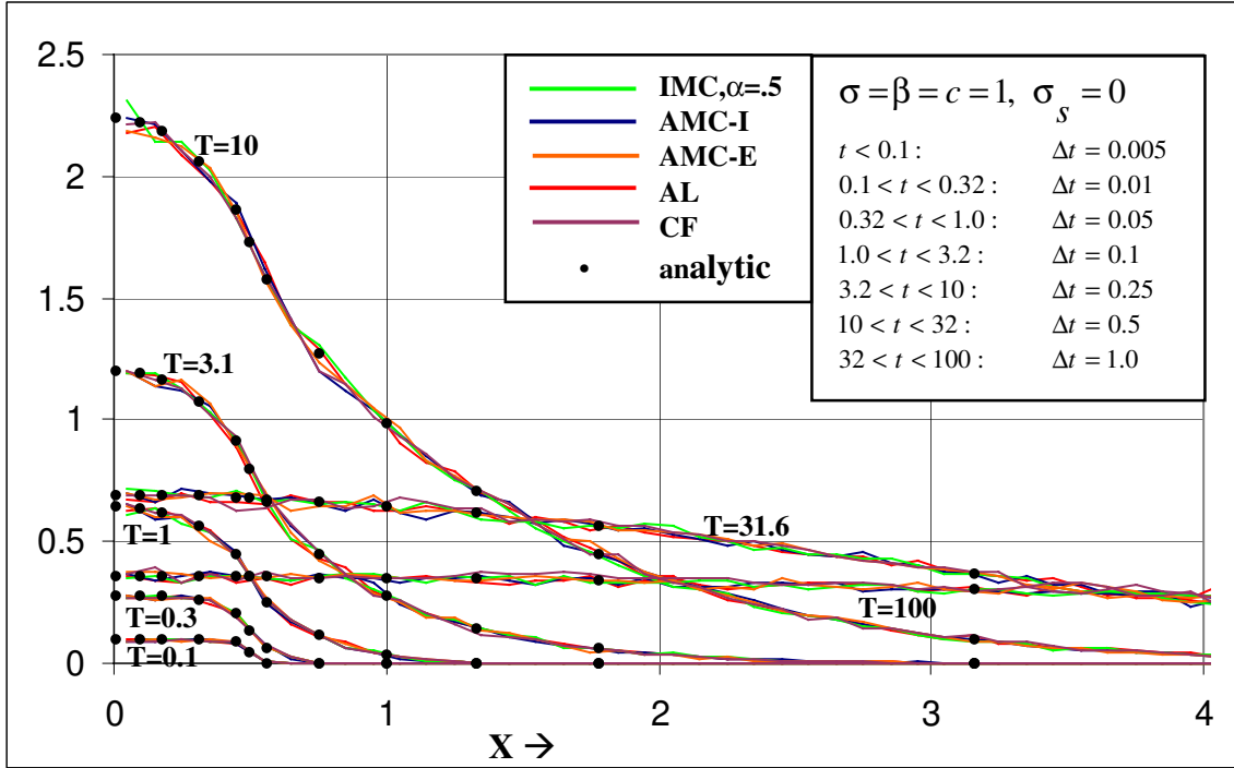
Figure 1. Integrated Radiation Intensity, \int I d\Omega , for Su-Olson problem, variable timesteps, \Delta t=5 , 100,000 source particles, 200 cells
