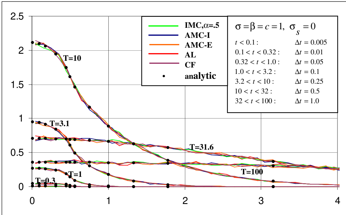
Figure 2. Equilibrium Radiation Energy Density, U_r , for Su-Olson problem, variable timesteps, 100,000 source particles, 200 cells
