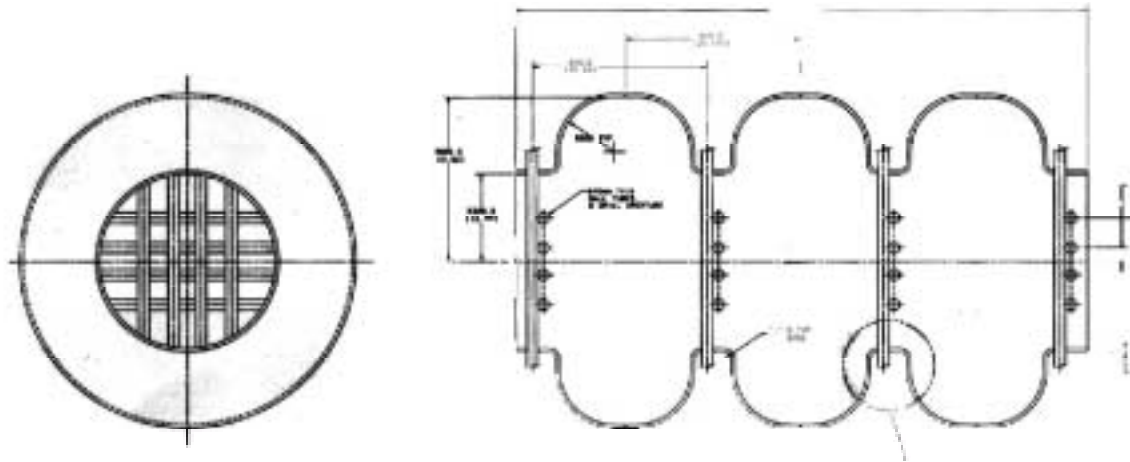
Fig. 5. Preliminary design of three-cell gridded NCRF cavity for 201 MHz operation.
