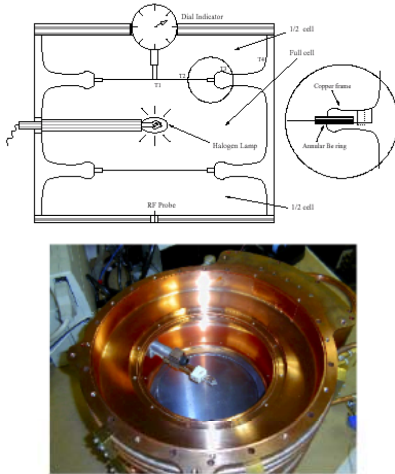
Fig. 2. (top) Schematic of Be window heating test setup with halogen lamp; (bottom) photograph of low-power pillbox cavity used for test.
