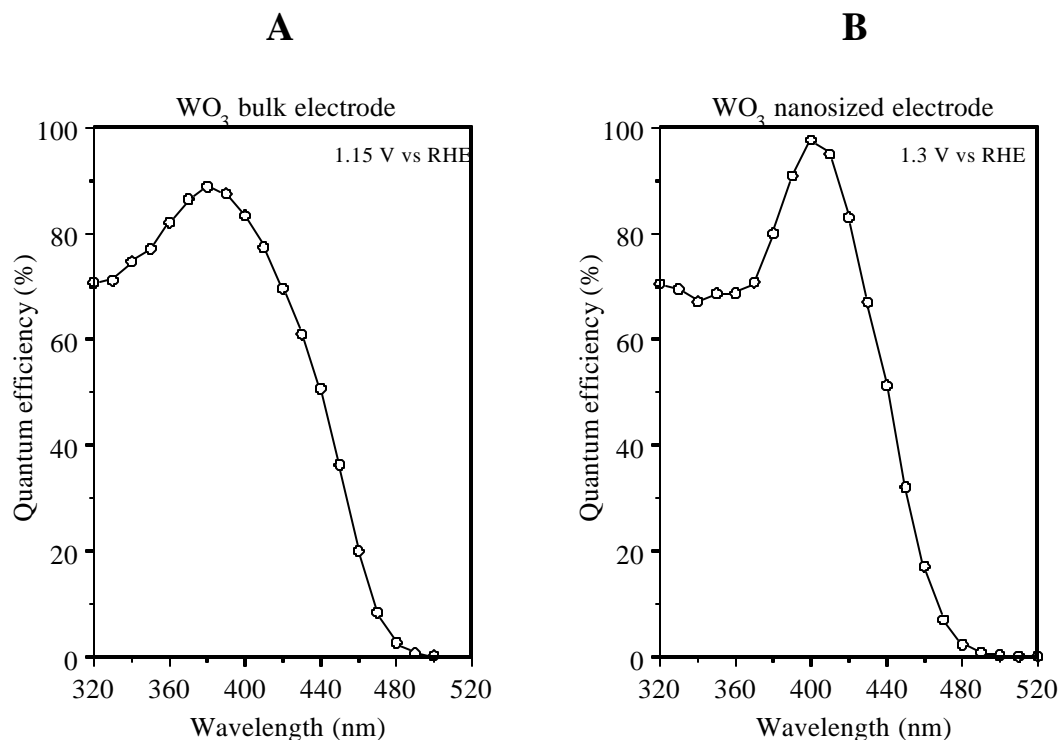
Figure 1: Spectral photoresponses associated with oxygen evolution at an activated bulk \text{WO}_3 electrode (A) and at a nanosized electrode (B) in 3M \text{H}_2\text{SO}_4 .
