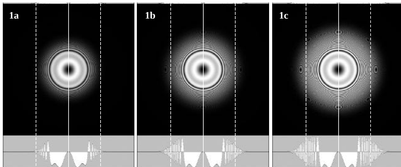
Figure 1. Conventional FEG-TEM. All plots show the CTF below a two-dimensional intensity spectrum. Dashed lines show 1 Å position. Plots for a CM300FEG-UT TEM with C_s=0.65\text{mm} at 300keV for a defocus of -430\text{Å} . (a) Typical mid-1990s spread of focus of \Delta=36\text{Å} , from an energy spread of 0.7eV FWHH and ripple of 1ppm, gives an information limit of 1.1Å. (b) CTF for NCEM one-Ångstrom microscope (OÅM) shows the current information limit of 0.78Å produced by a spread of focus of \Delta=20\text{Å} , computed from a measured 0.93eV FWHH. (c) CTF for a monochromated microscope with 200meV energy spread giving a spread of focus of \Delta=6.2\text{Å} and an information limit of 0.44Å.
