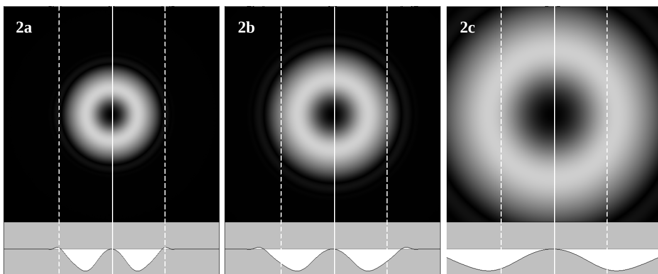
Figure 2. Optimum- C_s FEG-TEM. Plots for hypothetical C_s -corrected TEMs with C_s set at C_{s\text{opt}} = p^2\Delta^2/2 at 300keV. All plots show characteristic "donut" diffractograms with same-phase transfer out to crossover at the information limit. (a) Spread of focus of \Delta=36\text{Å} and information limit of 1.1Å. (b) For parameters (0.93eV FWHH) corresponding to those of the NCEM one-Ångstrom microscope (OÅM) a C_s -corrected TEM has same-phase transfer to 0.78Å. (c) A mono-chromated microscope with 200meV energy spread has same-phase transfer to an information limit of 0.44Å.
