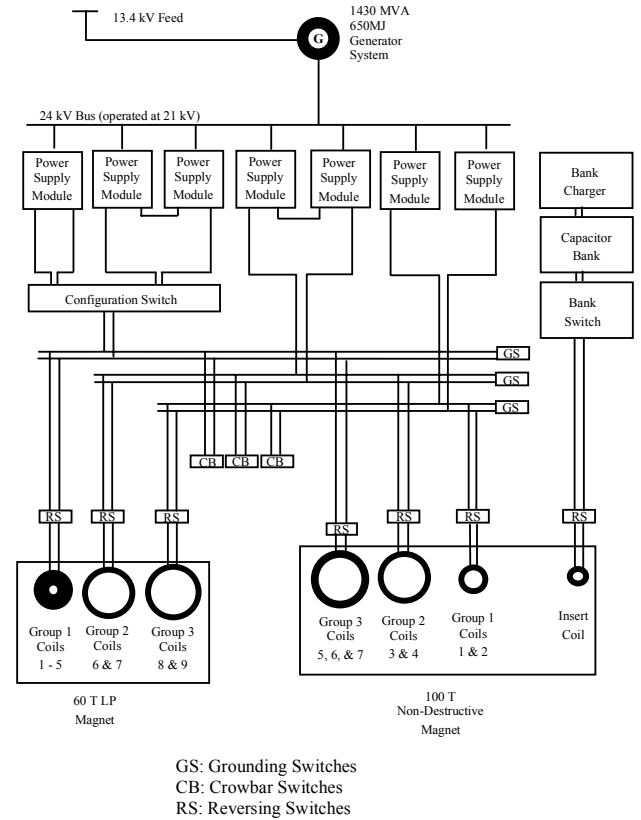
Fig. 3. 60 T LP/100 T ND Power Supply Schematic.
