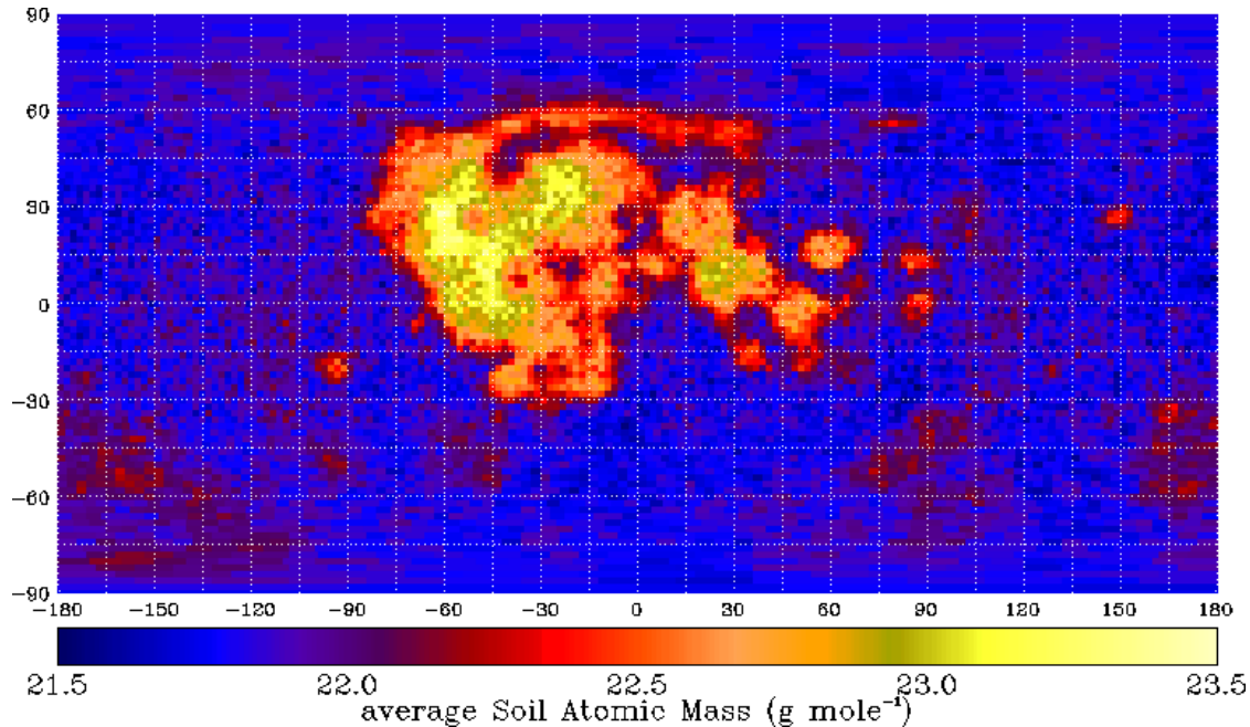
Figure 2. Approximative calibration of the fast neutron map as a measure of the average soil atomic mass \langle A \rangle .
