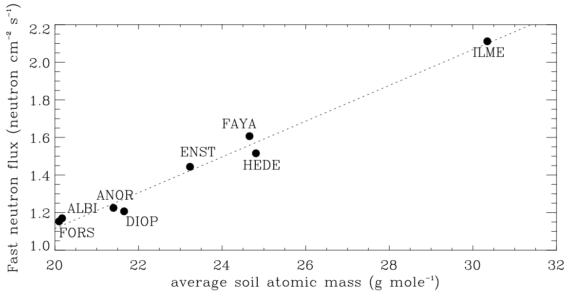
Figure 1. Integrated neutron leakage flux for compositions representing the poles of typical lunar minerals.
