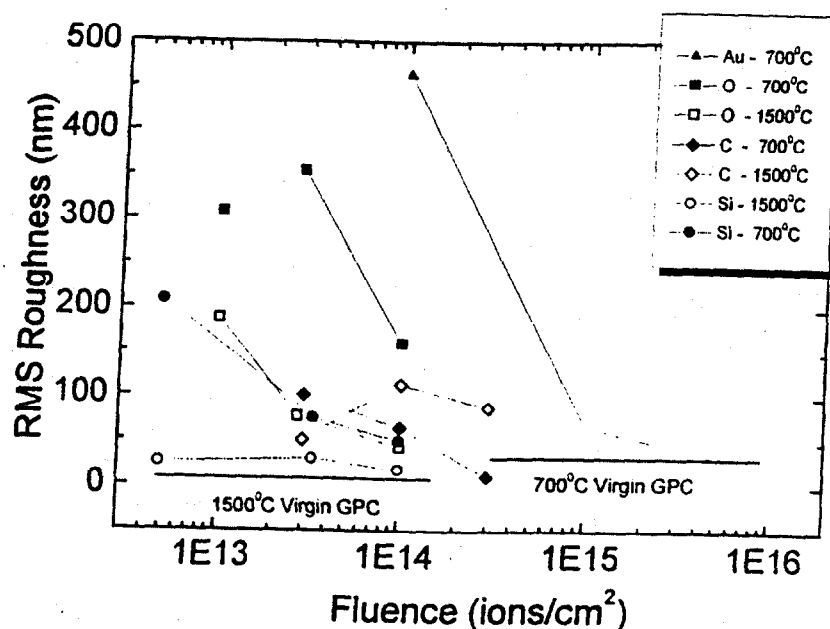
Fig. 3: RMS roughness of GPC as a function of fluence after bombardment with the ion shown. (See text for ion energies).
