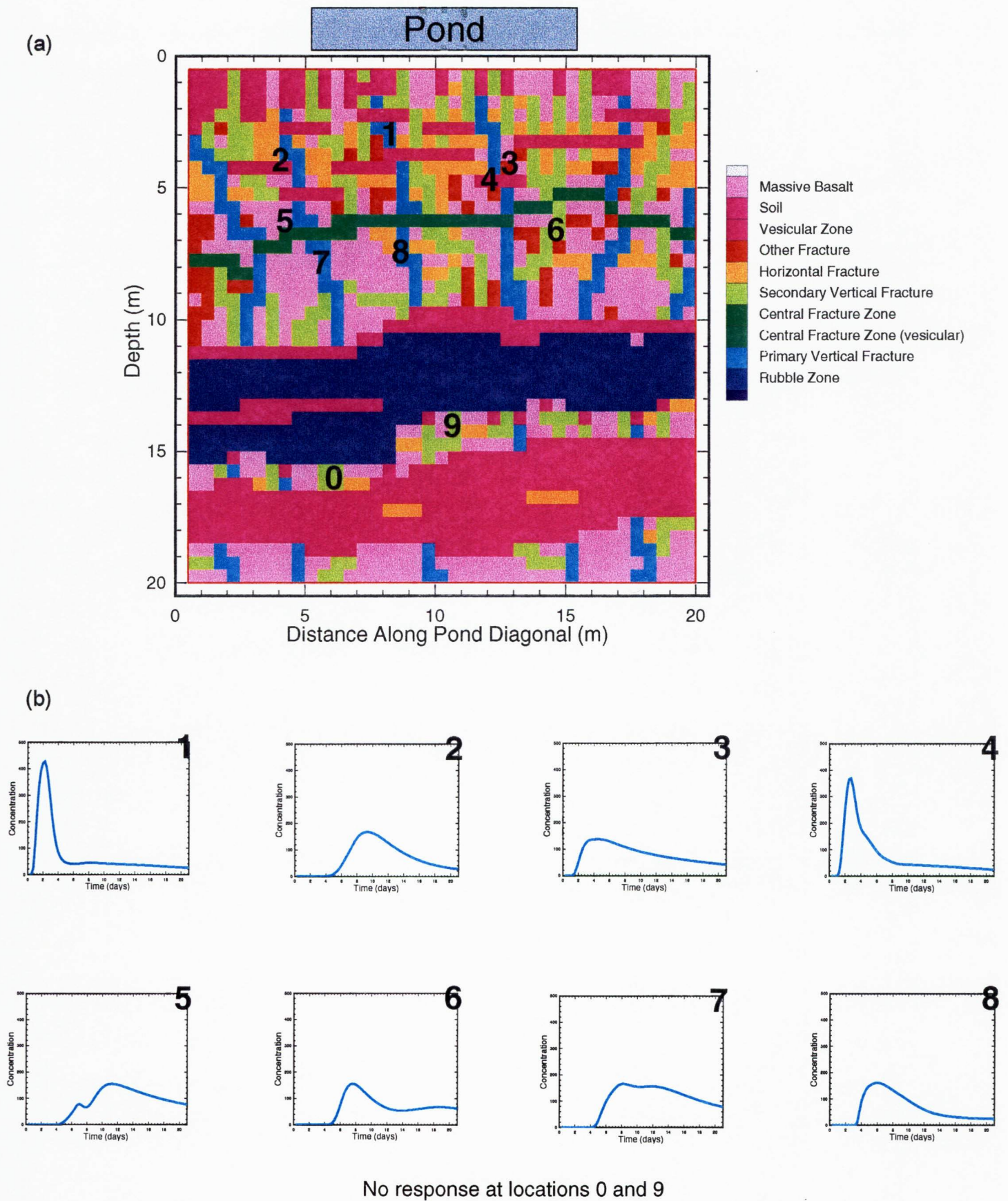
Figure 18. Numerical 2-D modeling of infiltration at the Box Canyon Site: (a) classification of rocks and soils, and (b) breakthrough curves corresponding to numbered locations in (a).
