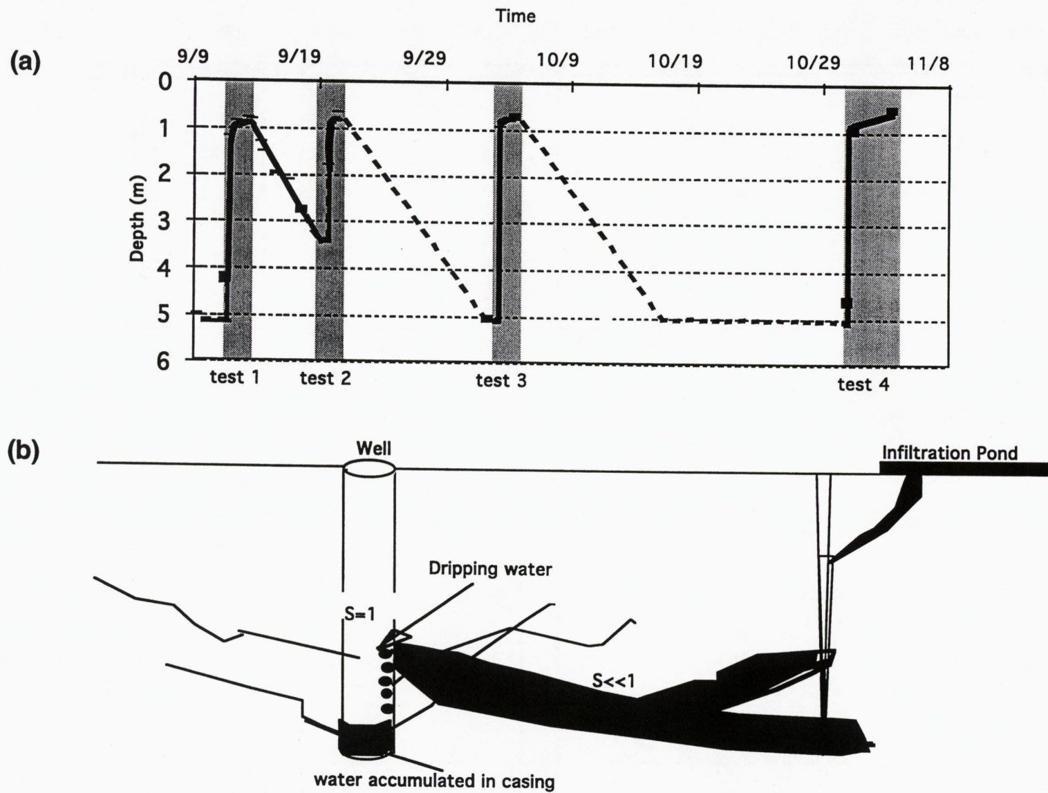
Figure 15. (a) Water level in well I-5 during the 1997 tests. The shaded areas indicate the time during which the surface was ponded; (b) Schematic diagram showing the creation of a water level in an open borehole in fractured rocks.
