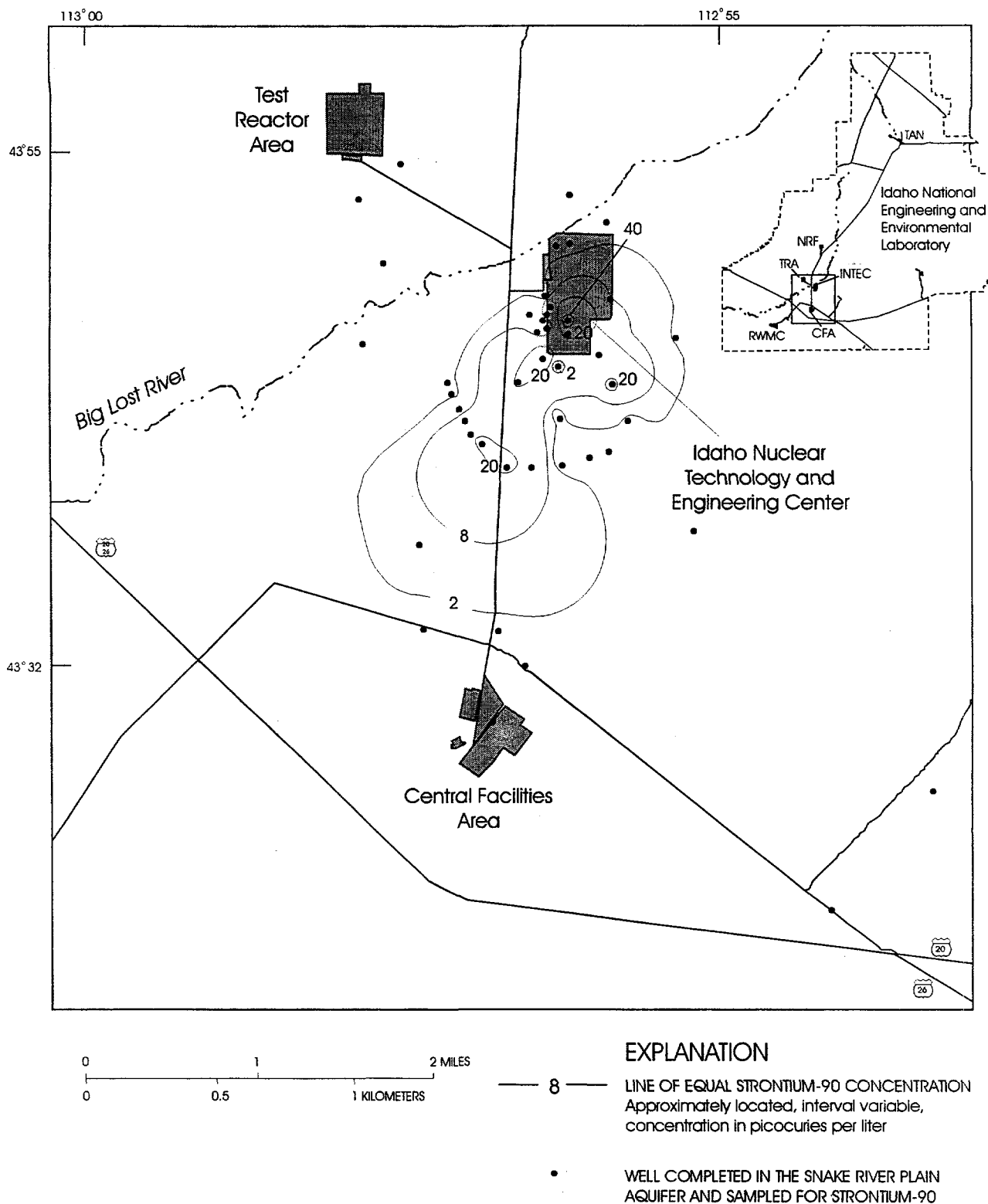
Figure 13. Distribution of strontium-90 in water from the Snake River Plain aquifer at the Idaho National Engineering and Environmental Laboratory, October 1998.
