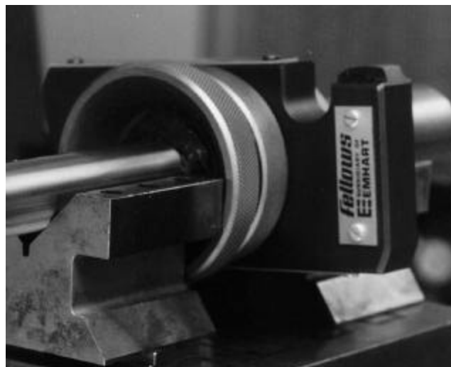
Figure 4 Involute Profile Artifact
