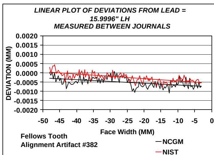
Figure 8 Inter-Comparison of Tooth Alignment Artifact
