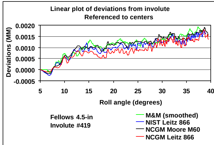
Figure 5 Inter-Comparison of Involute Profile Artifact
