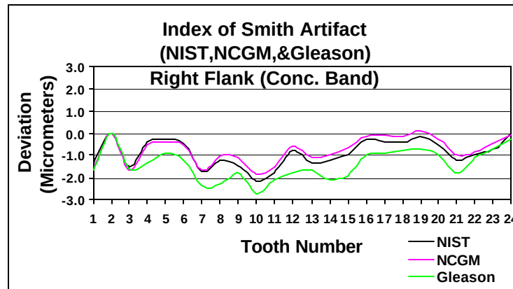
Figure 10 Inter-Comparison of Index Artifact
