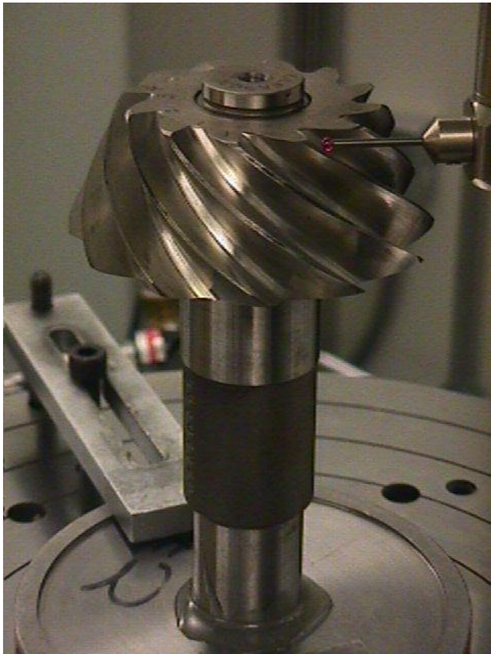
Figure 15 Bevel Pinion on Loan from Gleason
