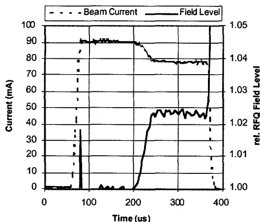
Figure 4: RFQ output current and field level versus time. RFQ nominal field level at ~97% of design.
