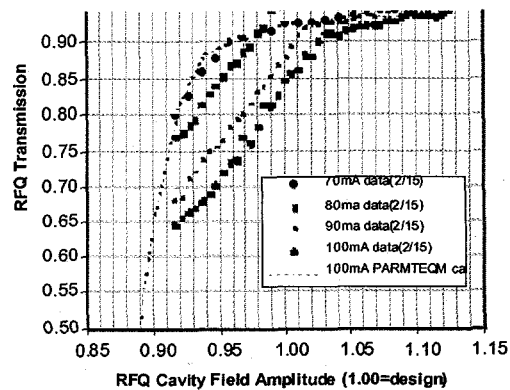
Figure 3: LEDA RFQ transmission data. Measurements performed at 70-100 mA peak current. PARMTEQM prediction for nominal 100-mA beam.
