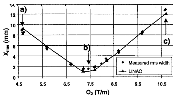
Figure 8. 93-mA x-scan data (diamonds) taken on three different days. The LINAC calculation (triangles, line) has Twiss parameters as described in the text.
