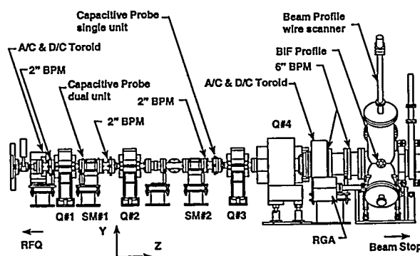
Figure 3. Layout of HEBT beamline optics and diagnostics. Beam direction is from left to right.
