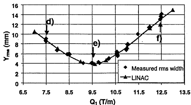
Figure 9. Same as Fig 8, except a y scan.
