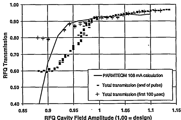
Figure 7. RFQ total and accelerated beam transmission vs. rf cavity field level at the start (crosses) and at the end (dashes) of a 500- \mu s-long, 90-mA beam pulse.
