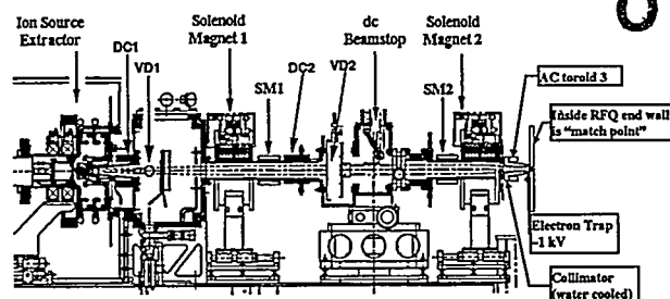
Figure 2. The LEBT beamline with optics and diagnostics.
