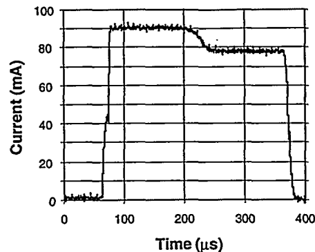
Figure 6. RFQ output beam current vs. time into a 300- \mu sec long pulse for the design RFQ rf-field level.
