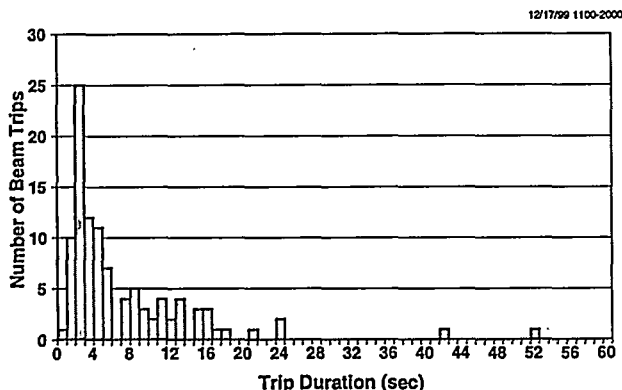
Figure 5. The number of beam trips vs. trip duration (data archived in 1 s intervals) for a 9-hr time period that includes the 3.3-hr interval displayed in Fig. 4.
