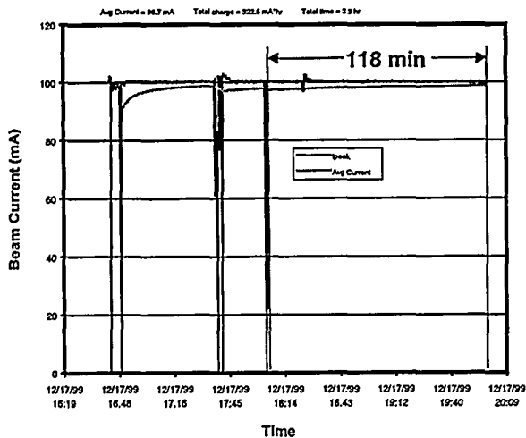
Figure 4. Archived RFQ output beam current (30-s intervals) for a 3.3 hr period on Dec. 17, 1999. Any beam interruptions during the last 118 min are <30-s long.
