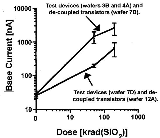
Figure 2 Comparison of high and low mode LM111 SPNP input transistor responses for room temperature 50 rad(SiO 2 )/s irradiations. Transistor distribution is similar to circuit.
