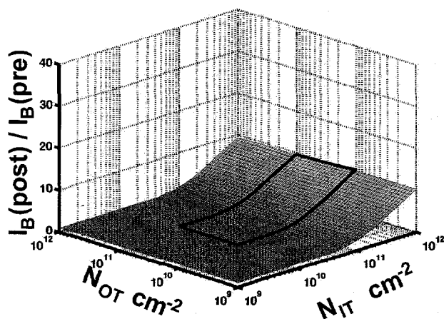
Figure 8 Normalized base current versus N_{OX} and N_{IT} for highly doped base ( 10^{17}\text{cm}^{-3} ) structure. Simulations indicate device sensitivity reduced by increased doping density.
