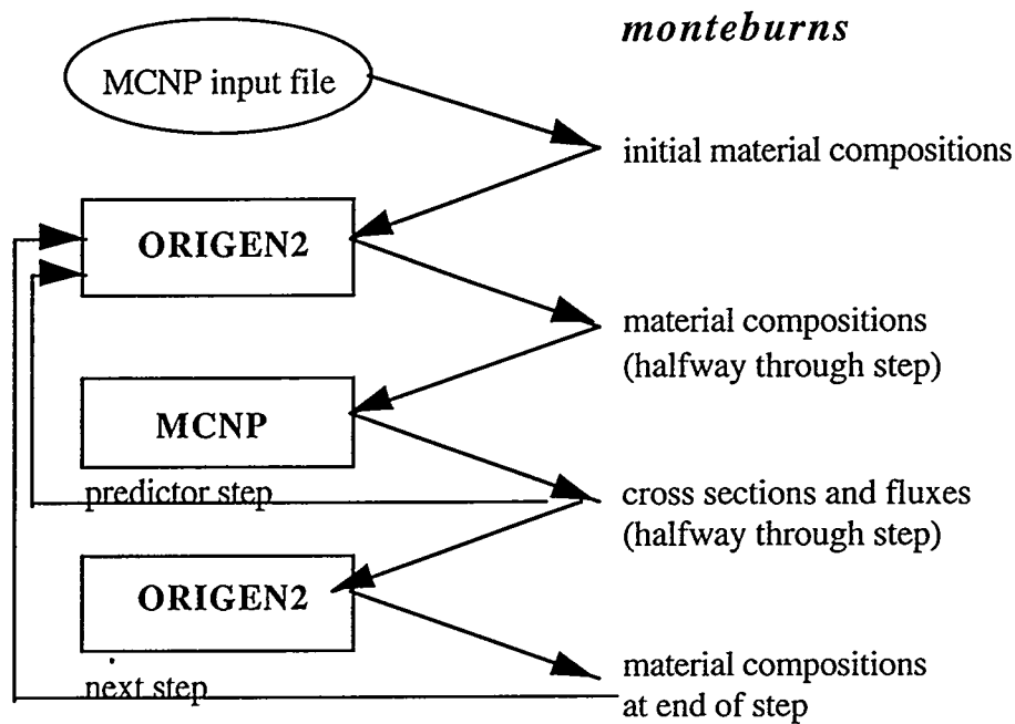
Fig. 1. Interaction of monteburns with MCNP and ORIGEN2.
