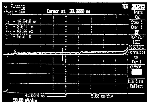
Figure 4: TDR reflection measurements.
