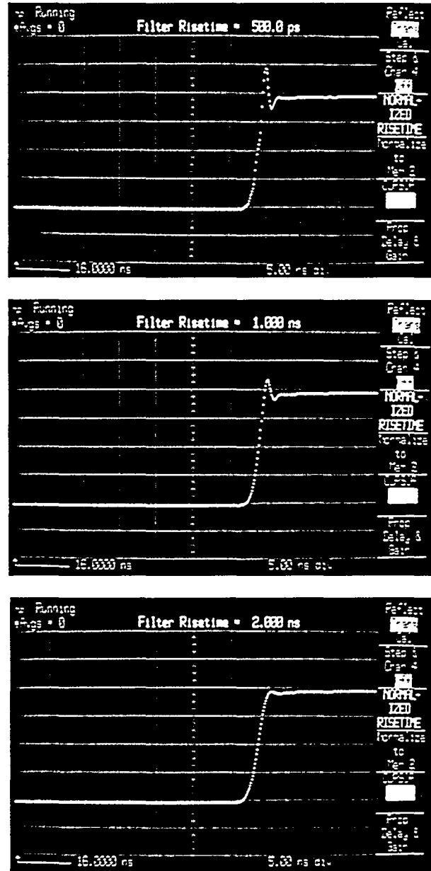
Figure 3: TDR transmission measurements using voltage pulses with fronts 0.5, 1, and 2 ns.
