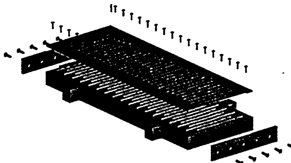
Figure 6: Exploded view of the 35-cm current structure assembly (courtesy of R.J. Roybal, LANSCE-1)
