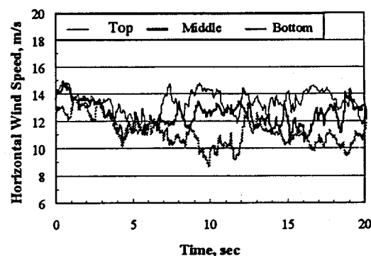
Fig. 9. Horizontal Wind Speed from the Bottom to the Top of the Rotor.
