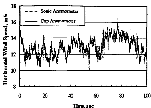
Fig. 5a. First 100 seconds of Data.
