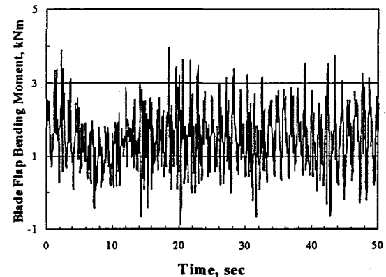
Fig. 17. Flap-Bending Moment at the 40 percent Span Location of Blade 2.
