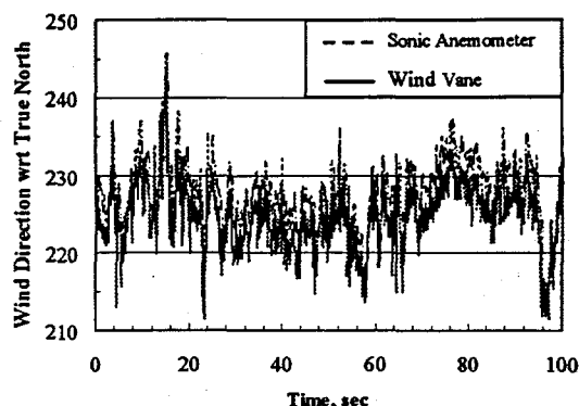
Fig. 6a. First 100 seconds of Data.
