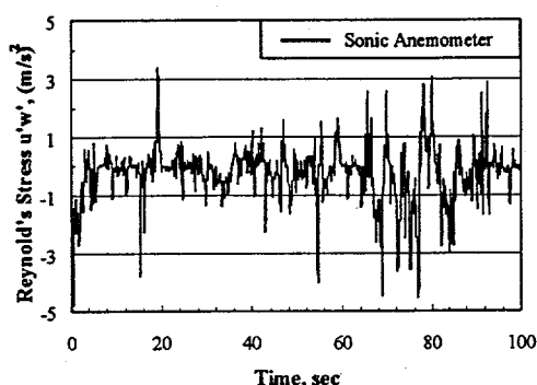
Fig. 8. Instantaneous Reynolds Stress for the Horizontal and Vertical Velocity Components.
