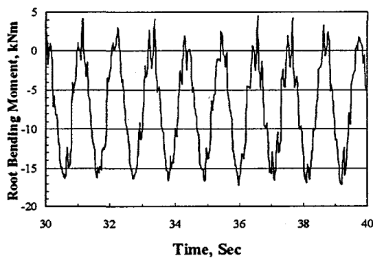
Fig. 14. Edge-Bending in the Root of Blade 1.
