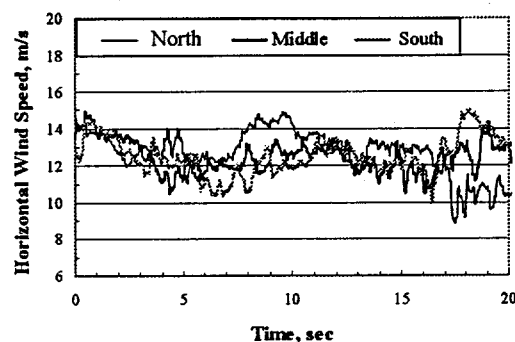
Fig. 10. Horizontal Wind Speed Across the Rotor Disk at Hub Height.
