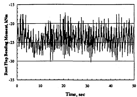
Fig. 16. Flap-Bending Moment in the Root of Blade 2.
