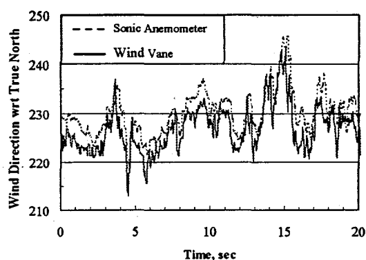
Fig. 6b. First 20 seconds of Data.
