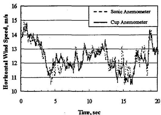
Fig. 5b. First 20 seconds of Data.
