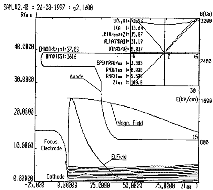
Fig.1 Simulation of extraction of the electron beam with current 13.64 A.
