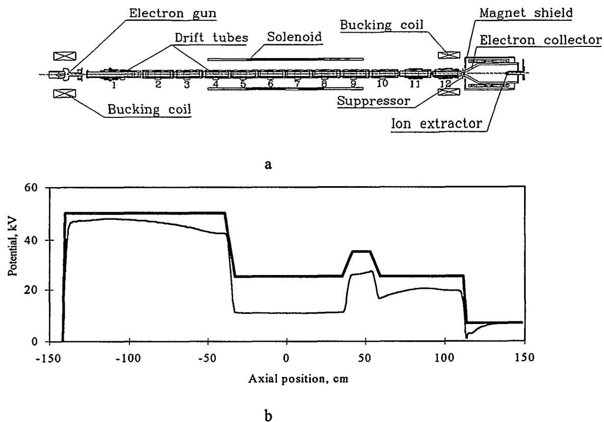
Fig. 3. A: Electron optical system of EBTS, b: Axial potential distributions on EBTS elements with constant drift tube inner diameters of 31 mm (solid line), and on the axis of a 13.64 A electron beam (fine line).
