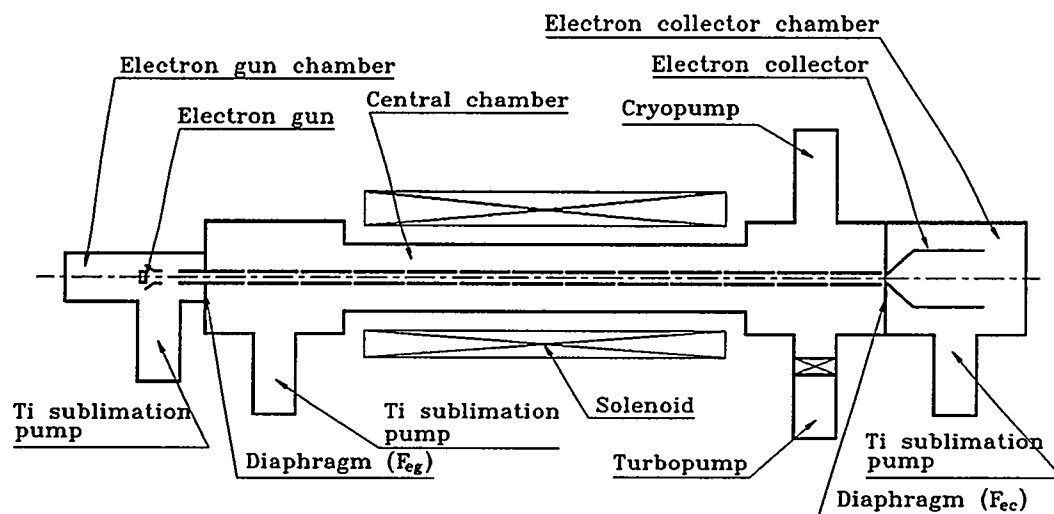
Fig. 4. Vacuum separation of the central region of the EBTS from the regions of the electron gun and electron collector. F_{eg} and F_{ec} are the vacuum conductivities of the electron gun chamber and electron collector chamber, respectively, with the central chamber.
