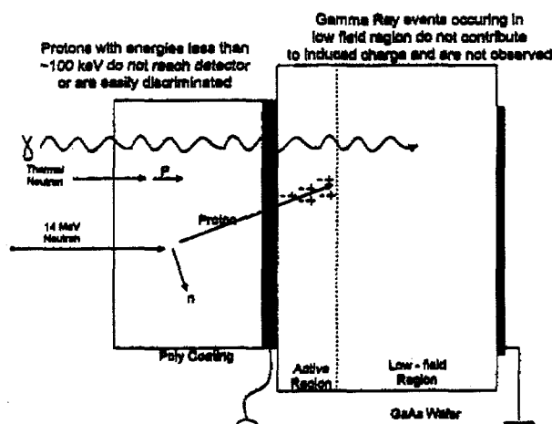
FIGURE 1. Schematic diagram of detector operation
