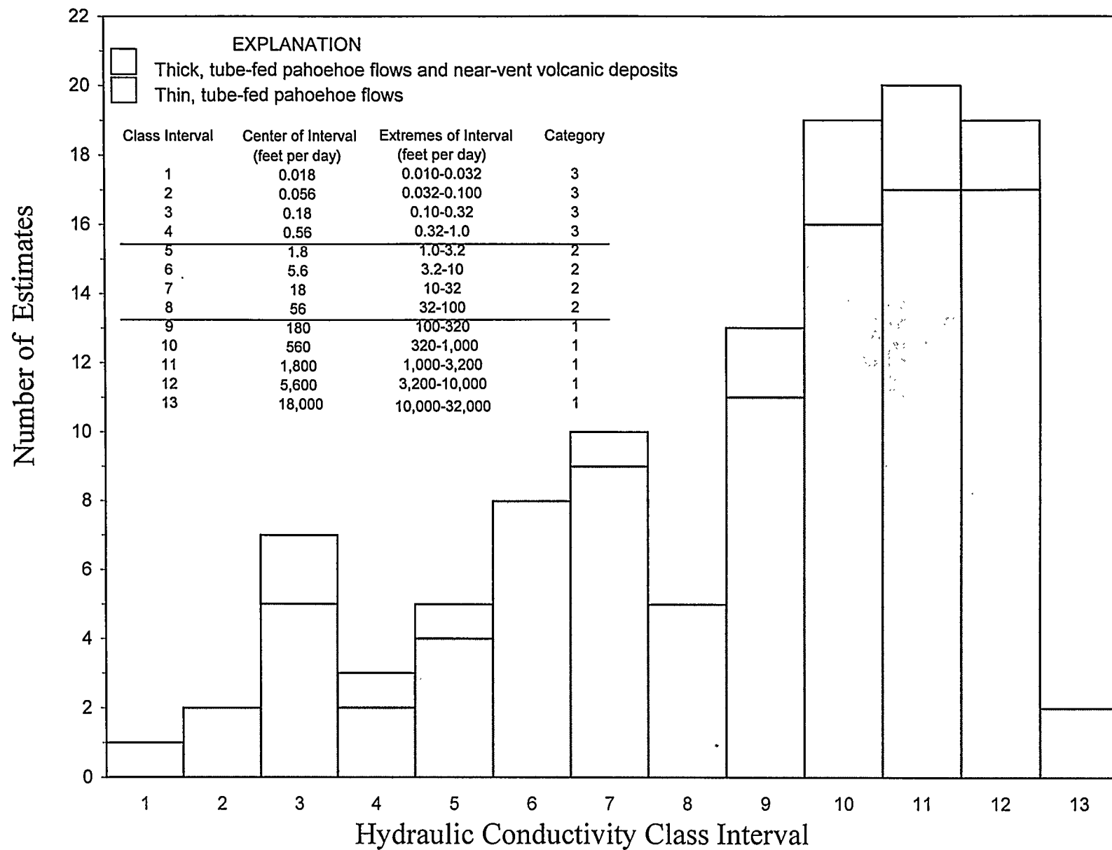
Figure 9. Frequency distribution of hydraulic conductivity estimates at and near the Idaho National Engineering and Environmental Laboratory (units are feet per day; range of intervals is 0.5 order of magnitude).
