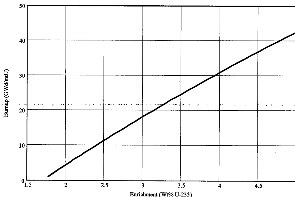
Figure 5. Preclosure Loading Curve for 0.929 Upper Subcritical Limit
