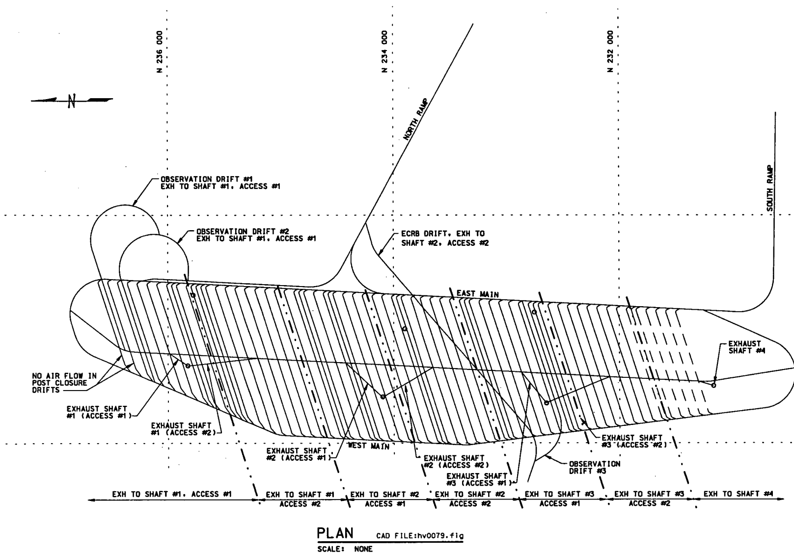
Figure 3. Exhaust Airflow Volume Allocations - 70,000 MTU Case
