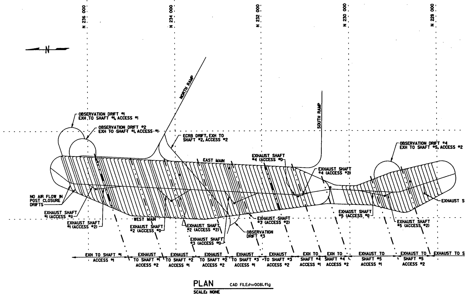
Figure 5. Exhaust Airflow Volume Allocations – 97,000 MTU Case
