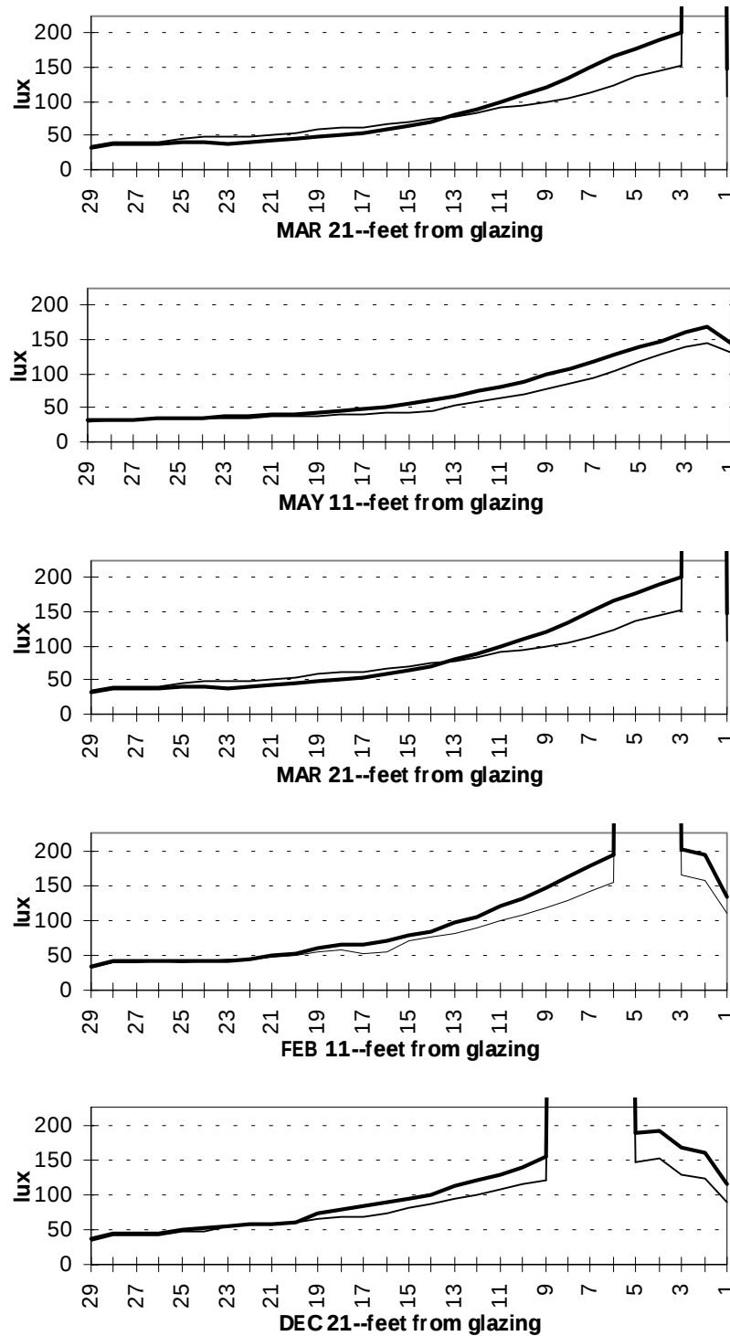
Figure 11. Illuminance distribution at 30 inches above the floor with holographic glazing with 75.6° acceptance and 18° diffraction angles (bold line) versus clear glazing (thin line).
