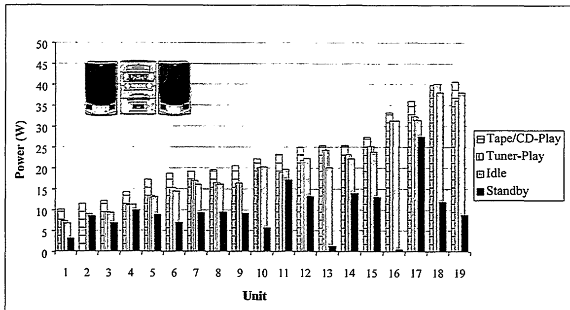
Figure 4-4. Measured Power Use of 19 Compact Stereo Systems in Standby, Tape/Line-Idle, CD-Idle, Tuner-Play, Tape-Play, and CD-Play Modes
