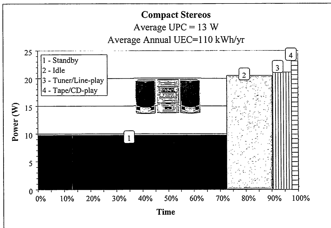
Figure 5-2. Average Power Requirements for Common Compact Stereo System Modes
