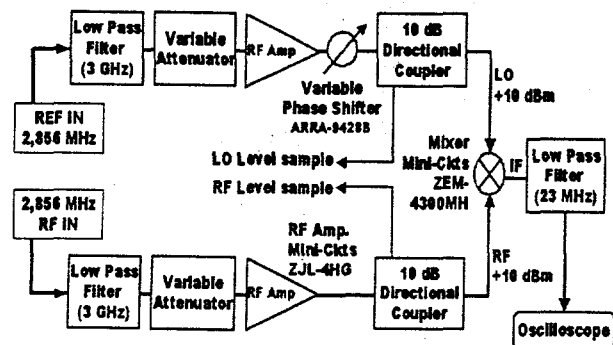
Figure 2: Block diagram of phase stability test unit.
