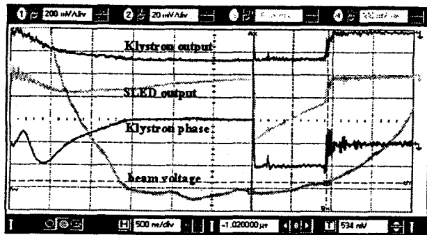
Figure 6: L2 after modulator trigger adjustments.
