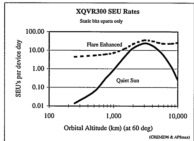
Figure 12: This plot is obtained by calculating the hypothetical sensitive volume of the XQVR300 as the product of all of the bits in the FPGA and the average cross-section from figures 3 and 4 earlier in this text. As demonstrated by the dynamic test data, the expected upset rate should be lower depending on the degree of mitigation employed.
