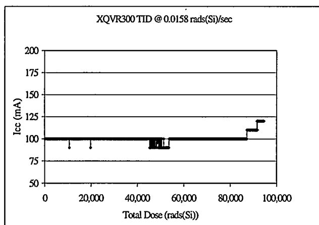
Figure 2: Low dose rate performance. In this case the increase in leakage current occurs above 90krads(Si) and does not constitute a failure below 100krads(Si).
