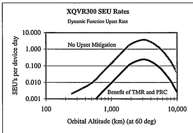
Figure 13: Applying the observed dynamic cross-sections to the upset rate calculations of the device, the maximum benefit observed so far in this work is plotted as the combined benefit of redundancy (TMR) and bitstream partial reconfiguration (PRC).
