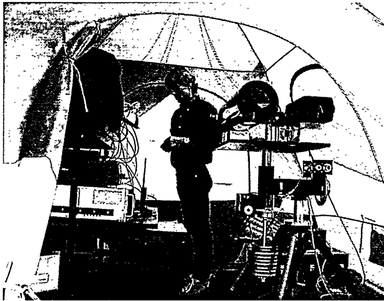
Figure 5. The free-space QKD receiver in operation.
