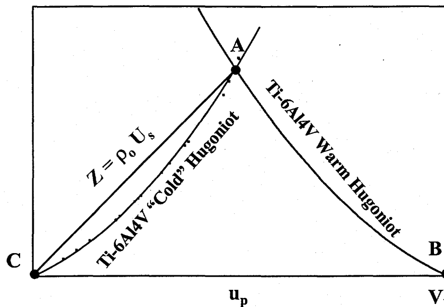
Figure 7. Pressure – particle velocity diagram. Ti-6Al4V Warm and Cold Hugoniot
