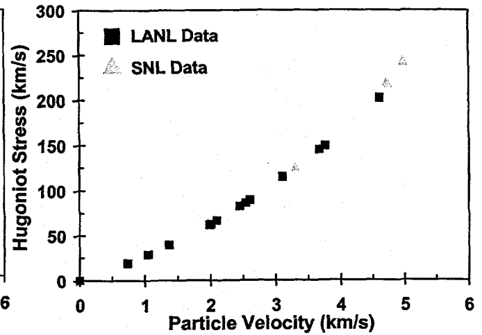
Figure 9. Pressure - particle velocity relationship
