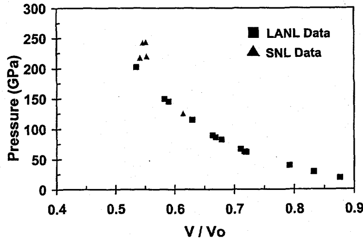
Figure 10. Pressure - Volume relationship
