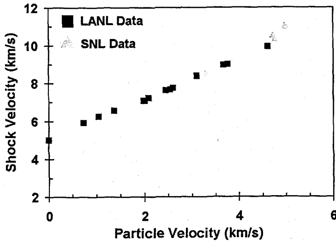
Figure 8. Shock velocity - particle velocity relationship
